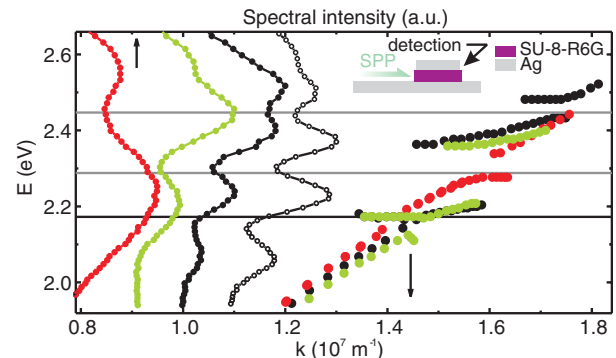
FIG. 3 (color online). The emission spectra measured from the waveguide samples having different lengths of R6G deposited on top of a waveguide (see the inset schematic), along with the dispersion curves of the thin film samples measured with DM2. The red, green, and black (or dark gray, gray, and black) spectra correspond to samples having 1, 2, and 5\ \mu\text{m} lengths of R6G, respectively. The spectrum with empty black circles is measured from a waveguide sample having a 5\ \mu\text{m} R6G area as well, but with a layer of silver deposited on top of this area (as in the schematic). In the dispersions red, green, and black (or dark gray, gray, and black) correspond to 4, 25, and 50 mM samples, respectively. The same color is used for pointing out the cases when the dips in the spectra and the splits in the dispersions appear at the same energies. The black horizontal line is the measured R6G emission and the gray lines absorption maximum and absorption shoulder energies.
