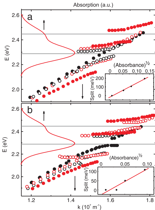
FIG. 2 (color online). The dispersions of four different samples having R6G concentrations of 4 mM (solid black circles), 25 mM (empty black circles), 50 mM (empty red or dark gray circles), and 200 mM (solid red or dark gray circles) measured by DM1 (a) and DM2 (b). The solid red or dark gray curves are the measured absorbance of the 200 mM SU-8-R6G film, and solid gray horizontal lines are the absorption maximum and absorption shoulder energies. The insets show the low (a) and high (b) energy splits as a function of (\text{absorbance})^{1/2} with linear fits.
