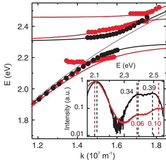
FIG. 4 (color online). The measured dispersions for 50 mM sample for DM1 (black) and DM2 (red or dark gray) and their theoretical fits. The solid gray curve is the theoretical dispersion of the uncoupled SPP on silver-SU-8 layer-air structure. The inset shows the normalized spectra for the 200 mM sample with DM1 (black) (background subtracted), and DM2 (red or dark gray), both with excitation light angle 71.5^\circ . The dashed lines show the spectral peak positions for the measurement methods DM1 (black) and DM2 (red or dark gray). The numbers indicate the intensity of the peaks.
