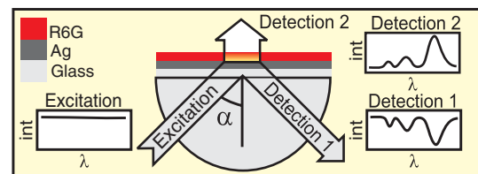
FIG. 1 (color online). The samples were studied by using three different, complementary detection methods. Detection 1 (DM1), applied before also, e.g., in Refs. [5,21,22], gives the energies that are coupled into the system as a function of in-plane wave vector k . The coupled modes are shown as dips in the reflected light. Detection 2 (DM2), not used in previous literature, gives the energies of the modes that are coupled out from the system by scattering processes. A third, waveguide-based method is introduced in Fig. 3.
