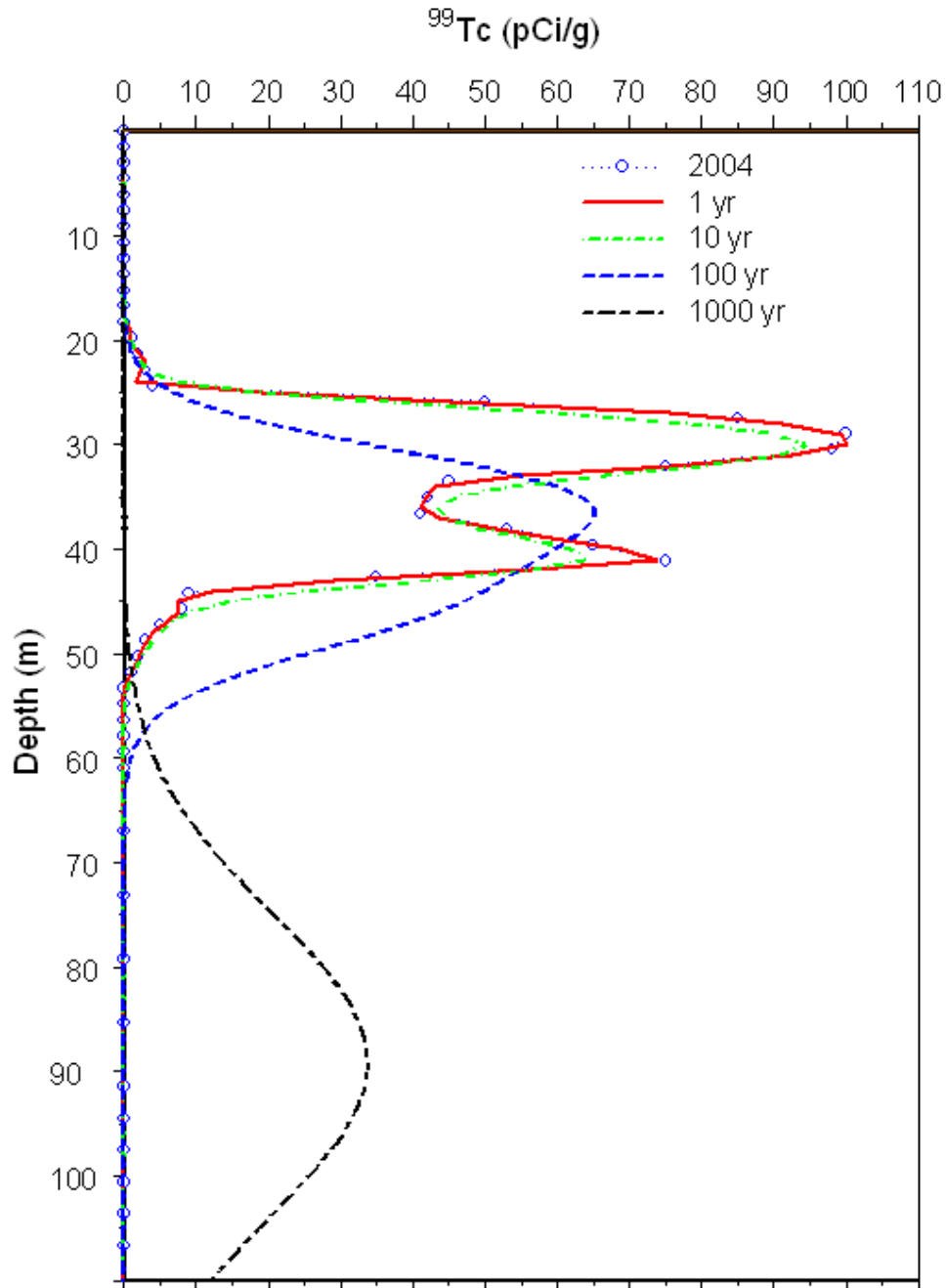
Figure 5.3. A Comparison of Measured and Predicted ^{99}\text{Tc} Concentrations Based on a 1-D Convolution Solution to the Convection-Dispersion Equation. The assumed recharge rate is 3.5 \text{ mm yr}^{-1} under the no-action alternative.
