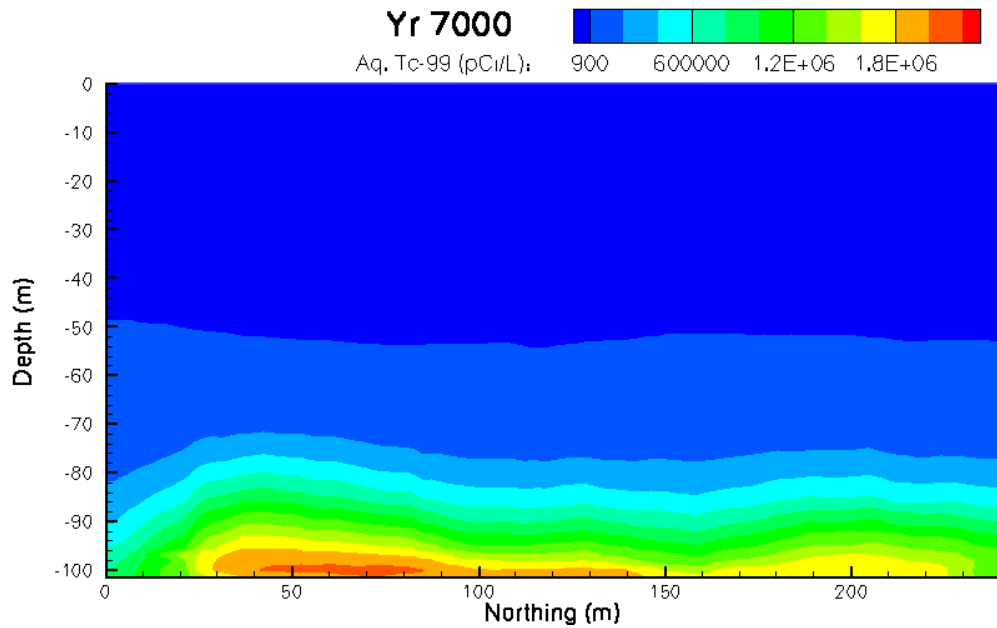
Figure 5.35. Calculated Distributions of Aqueous 99 Tc in the Year 7000 (0.1 mm/yr)
