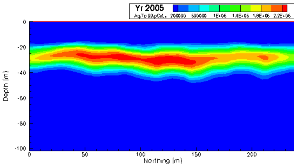
Figure 5.24. Calculated Distributions of Aqueous 99 Tc in the Year 2005
