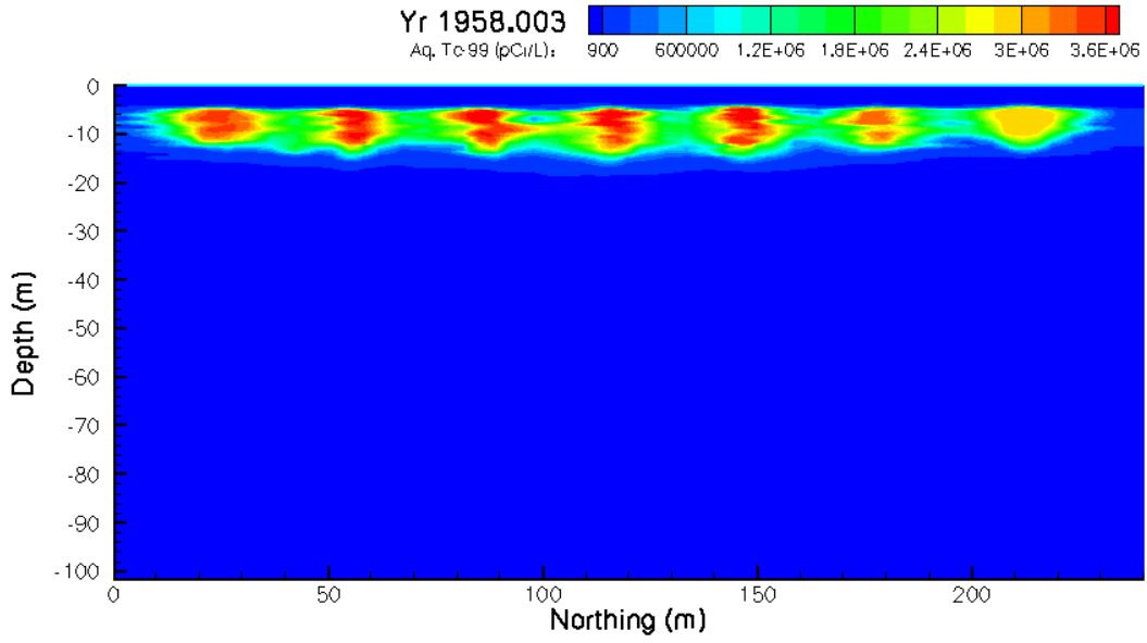
Figure 5.20. Calculated Distributions of Aqueous 99 Tc in the Year 1958.003
