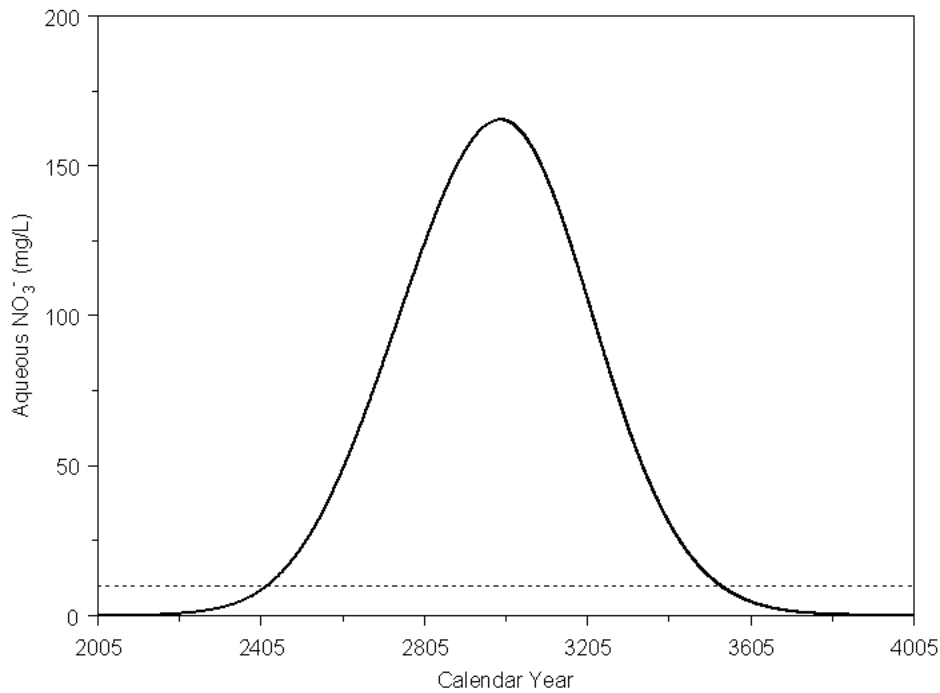
Figure 5.33. Calculated Distributions for NO 3 - at a Hypothetical Receptor well Under a Recharge Rate of 3.5 mm/yr based on STOMP Simulations. The dotted line is the MCL of 10 mg/L.
