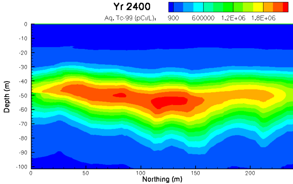
Figure 5.34. Calculated Distributions of Aqueous 99 Tc in the Year 2400 (0.5 mm/yr)
