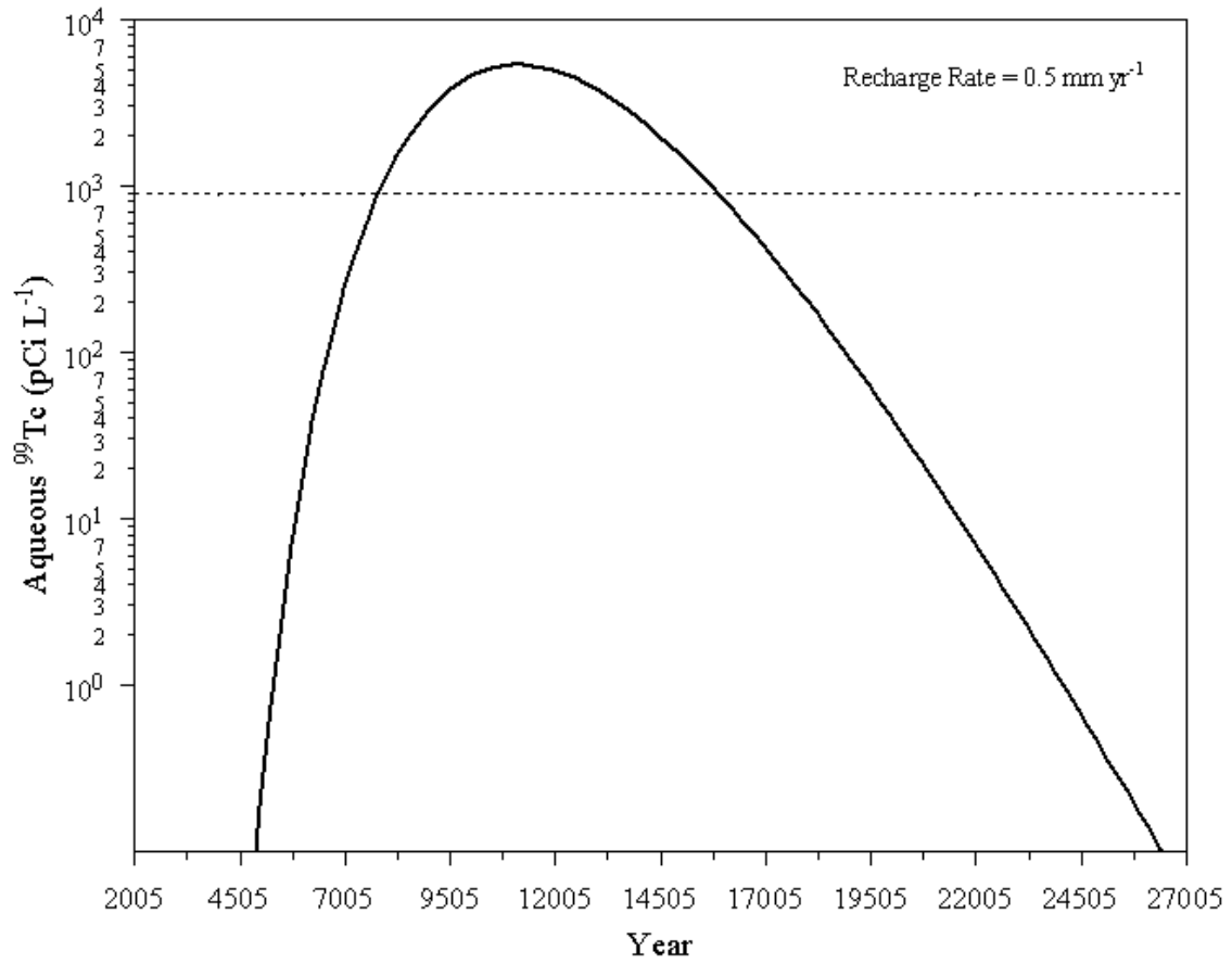
Figure 5.8. Calculated Distributions for 99 Tc at the Water Table Under a Recharge Rate of 0.5 mm/yr Using the 1-D Convolution Solution
