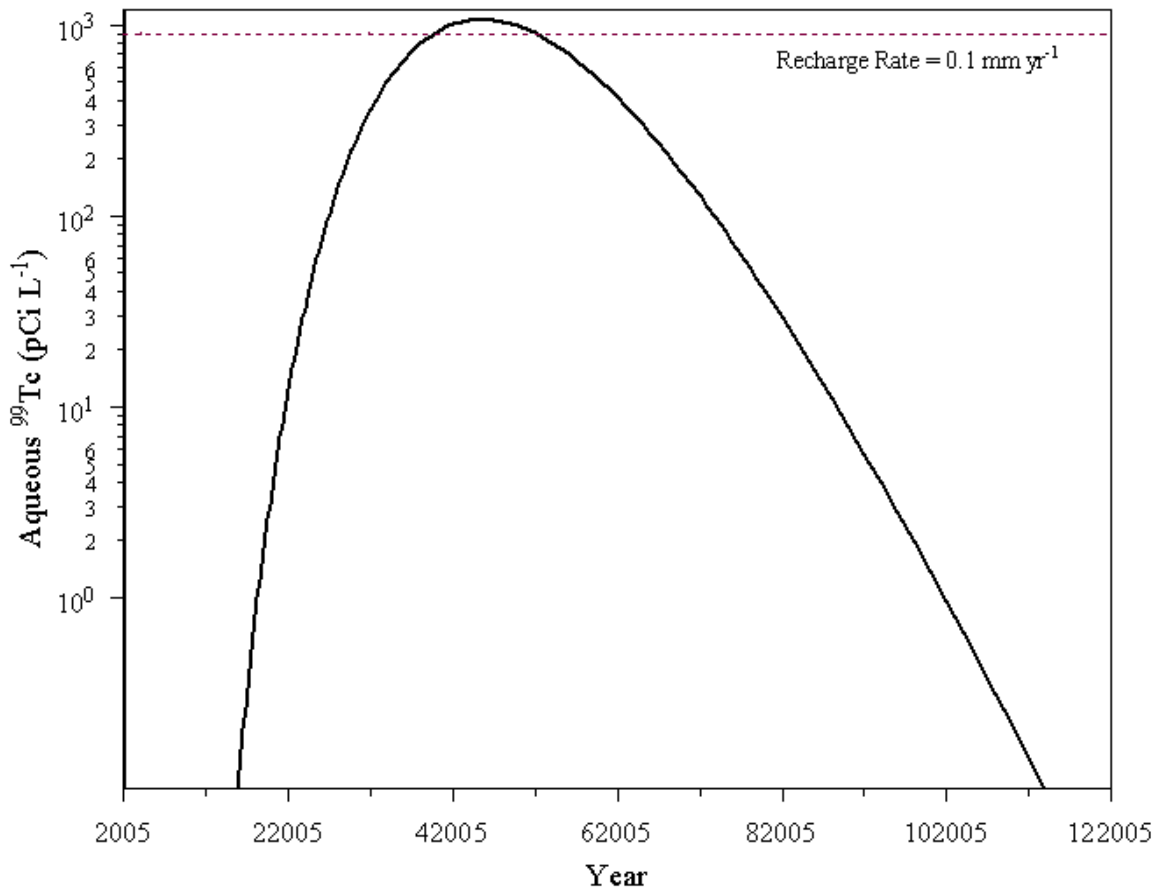
Figure 5.9. Calculated Distributions for 99 Tc at the Water Table Under a Recharge Rate of 0.1 mm/yr Using the 1-D Convolution Solution
