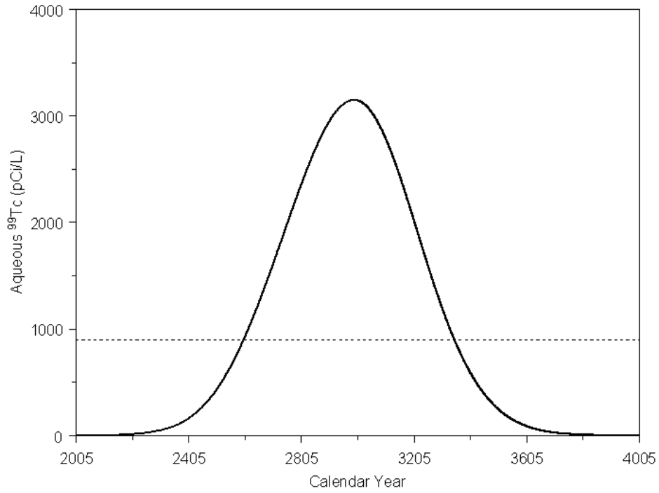
Figure 5.32. Calculated Distributions for 99 Tc at a Hypothetical Receptor well Under a Recharge Rate of 3.5 mm/yr based on STOMP Simulations. The dotted line is the MCL of 900 pCi/L.
