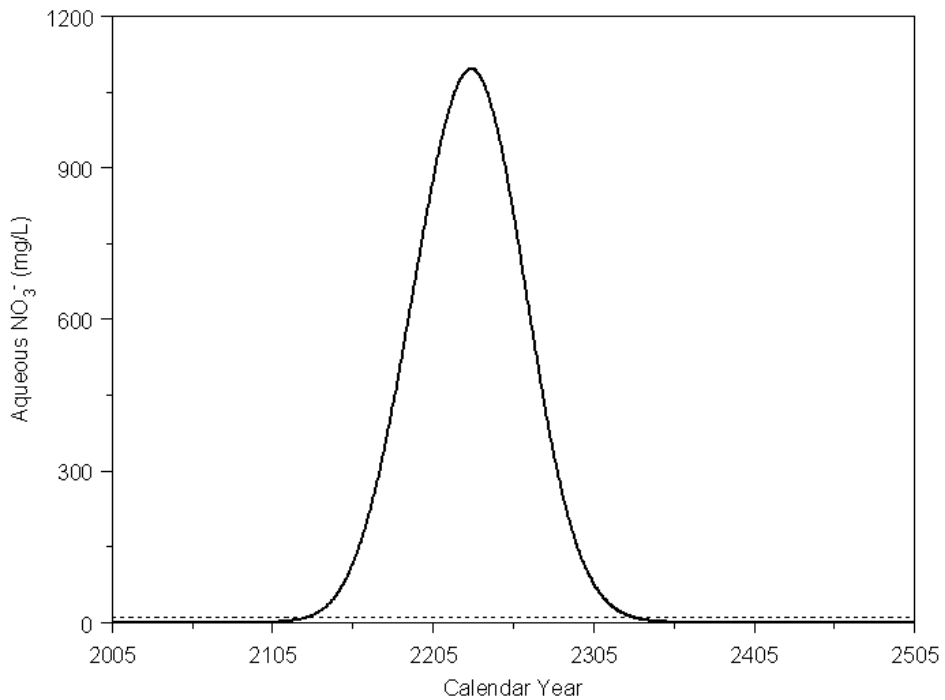
Figure 5.31. Calculated Distributions for NO 3 - at a Hypothetical Receptor well Under a Recharge Rate of 25 mm/yr Based on STOMP Simulations. The dotted line is the MCL of 10 mg/L.
