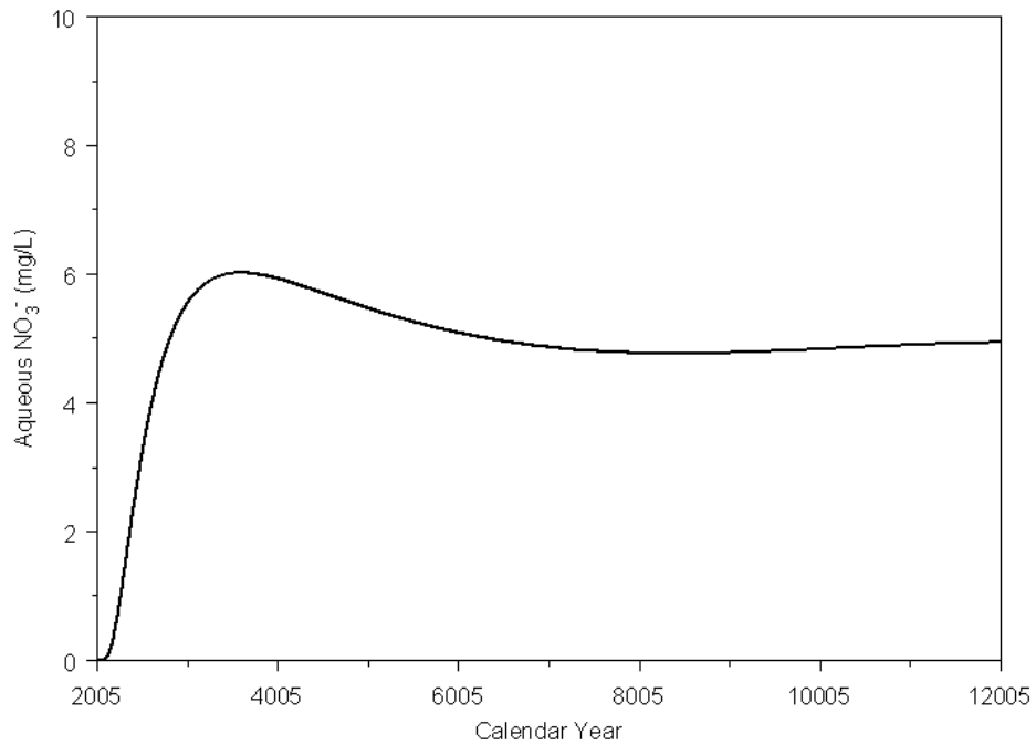
Figure 5.39. Calculated Distributions for NO 3 - at a Hypothetical Receptor well Under a Recharge Rate of 0.1 mm/yr Based on STOMP Simulations
