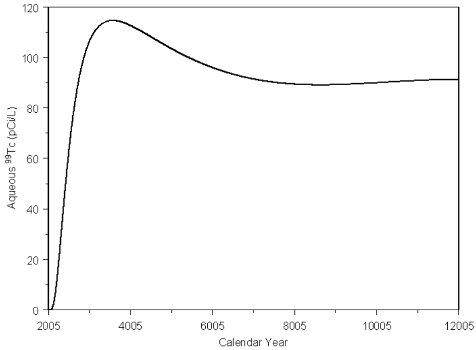
Figure 5.38. Calculated Distributions for 99 Tc at a Hypothetical Receptor well Under a Recharge Rate of 0.1 mm/yr Based on STOMP Simulations
