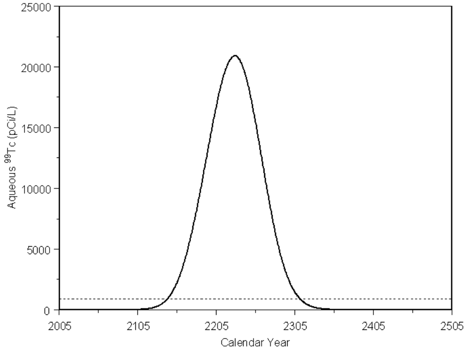
Figure 5.30. Calculated Distributions for 99 Tc at a Hypothetical Receptor well Under a Recharge Rate of 25 mm/yr Based on STOMP Simulations. The dotted line is the MCL of 900 pCi/L.
