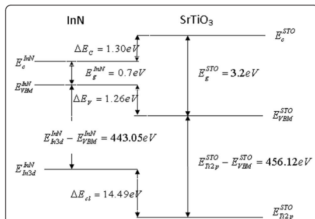
Figure 2 Schematic representation of the band line-up at an InN/SrTiO 3 heterojunction at the room temperature. A type-I heterojunction is formed in the straddling configuration.
