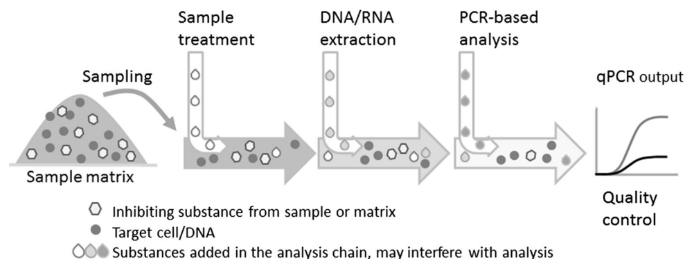
Fig. 6 Sources of matrix effects in PCR. The sample flow in the PCR analysis chain is shown. Substances that disturb PCR (i.e. PCR inhibitors) may be added to the samples in any of the modules. The
