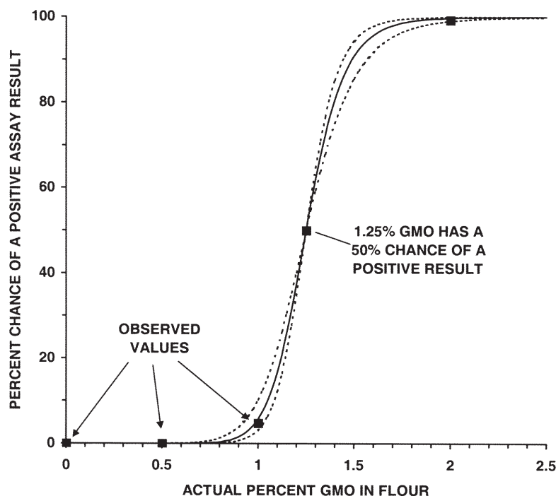
Figure 1. Predicted assay sensitivity to actual levels of GMO in soybean flour. Dashed lines indicate 95% confidence limits on the sensitivity curve.
