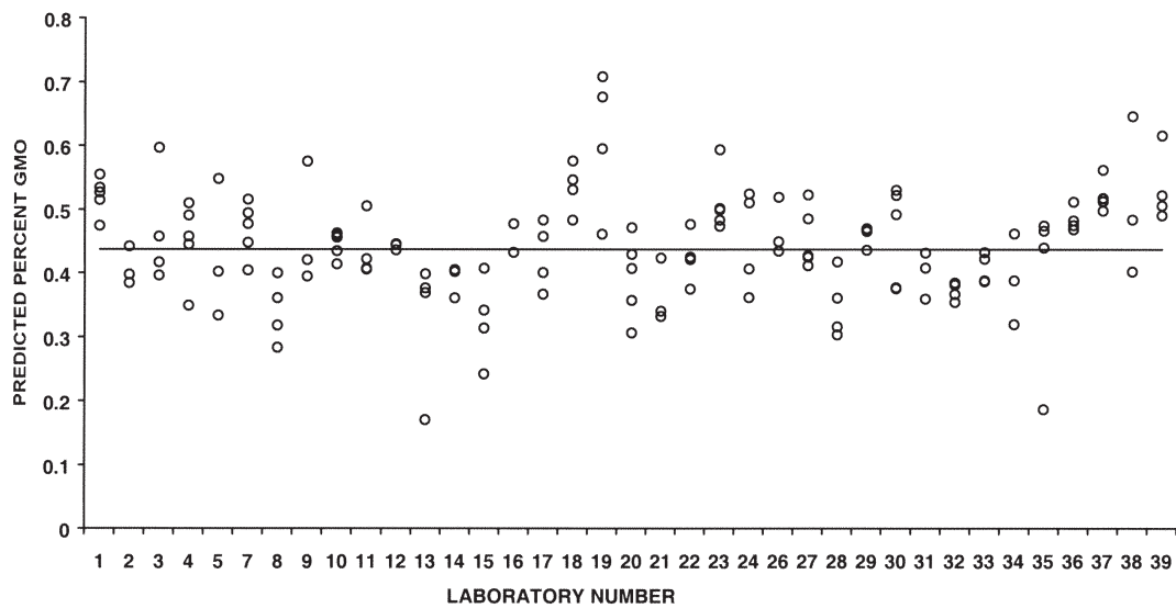
Figure 2. Summary of 0.5% GMO sample results for all laboratories. Horizontal line is median computed for all data.
