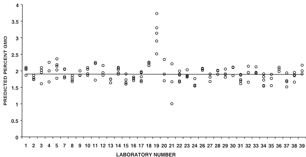
Figure 4. Summary of 2% GMO sample results for all laboratories. Horizontal line is median computed for all data.
