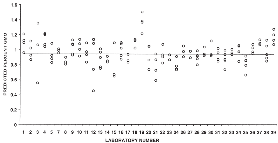
Figure 3. Summary of 1% GMO sample results for all laboratories. Horizontal line is median computed for all data.
