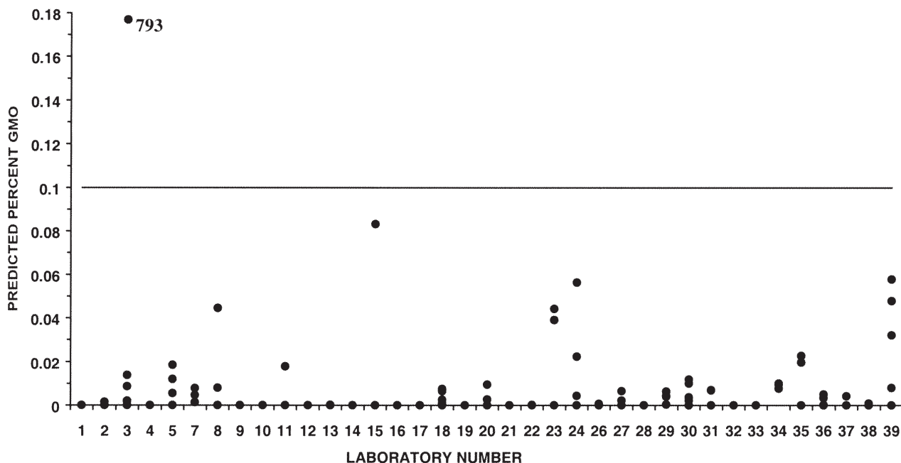
Figure 5. Summary of 0% GMO sample results for all laboratories. All samples yielding a noncomputable value were set equal to 0% GMO. Horizontal line is proposed detection criterion.
