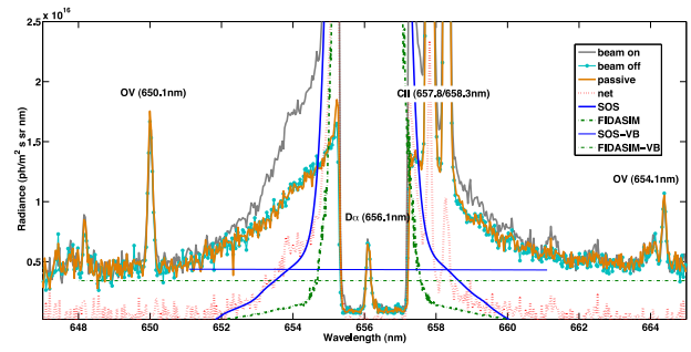
FIG. 3. The FIDA spectrum from a poloidal LOS at r/a \sim 0.1 : (1) measured spectra: including both active and passive components during the probe beam on (“beam on”), passive spectra during the beam off (“beam off”), passive spectra from the pair N-port passive viewing (“passive”), active FIDA radiation (“net”) with the subtraction of “beam off” from “beam on”; (2) calculated spectra: from SOS and FIDA simulations excluding bremsstrahlung part (“SOS,” “FIDA”), and each bremsstrahlung calculations (“SOS-VB,” “FIDA-VB”). The intensity of the cold D_\alpha line have been attenuated by the neutral density filter placed in the focal plane between the spectrometer and camera.
