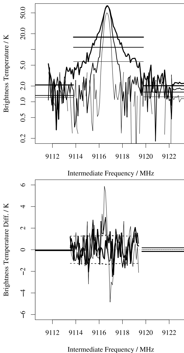
Figure 3. (top) Radiances and (bottom) residuals (measured radiances – calculated radiances) for DACS band 25. All quantities are mean daily values for a 10^\circ latitude bin centered at 80^\circ\text{N} . The lines are for tangent heights of 50 km (thick), 65 km and 80 km (thin). Channels 12–14 of band 9 are also visible in the plot. Note that residuals are shown only for channels that are used in the retrieval: Channel 13 of band 9 is not used as the DACS makes the information it would provide entirely redundant. DACS channels are not used where they overlap band 9 channels 12 and 14. The dashed lines are the expected 1\text{-}\sigma random error in this average, that is, the random error on a single measurement divided by the square root of the number of profiles in the latitude bin. The residuals exceed this near the line center, where there is a noticeable Doppler shift caused by wind that is not modeled. The target CO line appears at an intermediate frequency of 9117 MHz.
