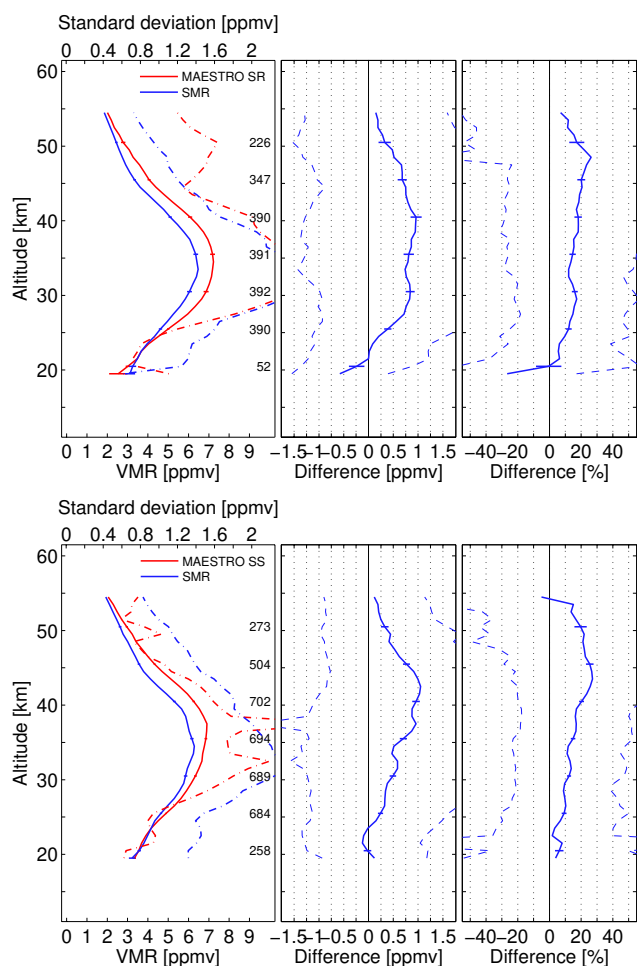
Fig. 12. Same as Fig. 1, but for the comparisons between ACE-MAESTRO and SMR. Top: comparison with ACE-MAESTRO SR observations; bottom: comparison with ACE-MAESTRO SS observations.
