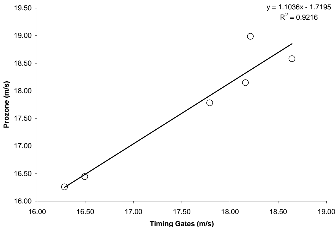
Figure 7. Relationship between the actual velocity of the subject measured by timing gates vs that calculated by Prozone® camera system during the 20m sprint and turn test. (n=6).
