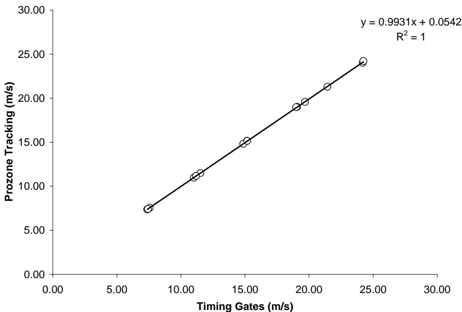
Figure 4. Relationship between the actual velocity of the subject measured by timing gates vs that calculated by Prozone® camera system during the 60m running test. (n=3, 5 different velocities measured).
