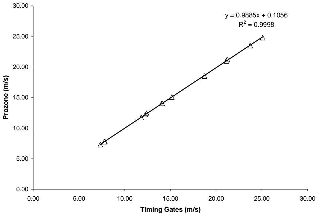
Figure 5. Relationship between the actual velocity of the subject measured by timing gates vs that calculated by Prozone® camera system during the 50m curved running test. (n=3, 5 different velocities measured).
