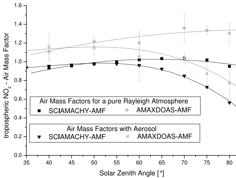
Fig. 4. The AMF for both instruments SCIAMACHY and AMAXDOAS. In general AMAXDOAS is more sensitive to tropospheric pollution than SCIAMACHY. The \text{NO}_2 was assumed to be well mixed within the boundary layer (1 km) and to decrease to 0 within the next km. For the aerosol case, a visibility of 4.8 km and an urban aerosol type was assumed in the boundary layer.
