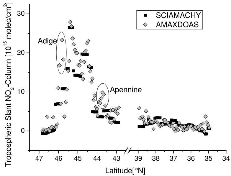
Fig. 8. Slant \text{NO}_2 columns measured by SCIAMACHY and AMAXDOAS. In the gaps between two SCIAMACHY Nadir scans no data are shown.
