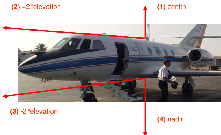
Fig. 2a. Pictures of the DLR-Falcon, including a sketch of the used lines of sights.
