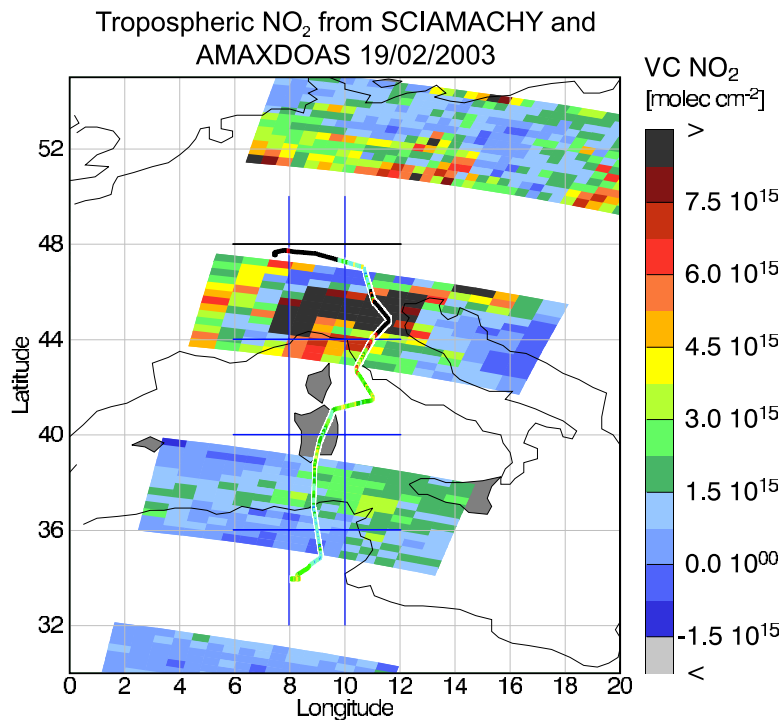
Fig. 7. Tropospheric vertical NO 2 column measured by AMAXDOAS and SCIAMACHY. The AMAXDOAS data were overlaid over SCIAMACHY's pixel in the same scale using similar colours. Zürich is not covered by SCIAMACHY's pixel on this.
