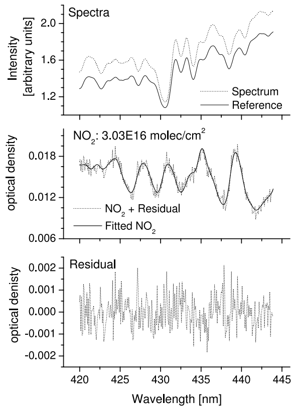
Fig. 3. \text{NO}_2 -fit for a Nadir spectrum, the measurement was done on the flight on 19/02/2003 from Basel to Tozeur at 08:14:30 UT close to Zürich, the reference was taken about 15 min later in the clean air of the Alps.
