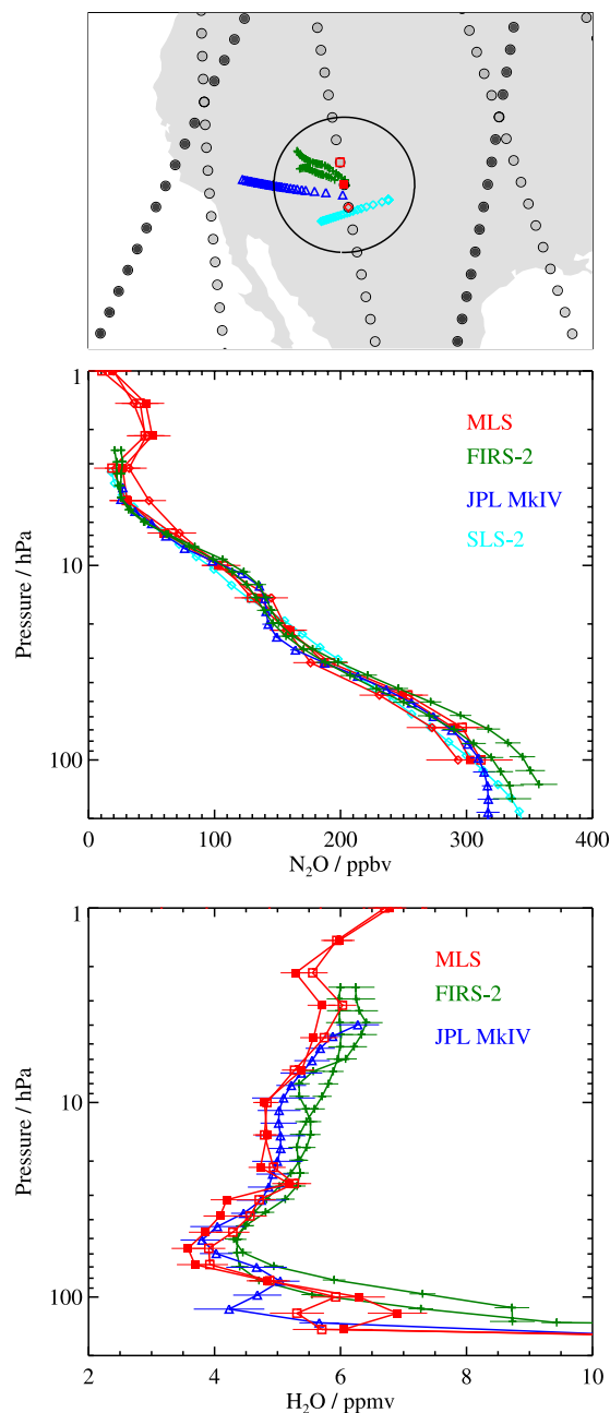
Figure 27. MLS N 2 O and H 2 O ascending orbit overpass measurements (20 September, 2027 UT) compared to the FIRS-2 (20 September, 2034 and 2144 UT), JPL MkIV (21 September, 0043–0147 UT) and SLS-2 (20 September, 1750 UT) measurements from the BOS gondola flown from Fort Sumner on 20–21 September 2005. Horizontal error bars indicate the 1-sigma precisions. Location map details are as in Figure 24 except an additional MLS profile match (red diamond symbol) for N 2 O is shown which matches better the SLS-2 measurement locations.
