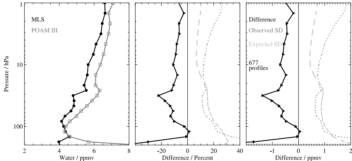
Figure 18. As Figure 13 except for POAM III H 2 O averaged over 92 d of collocated data.
