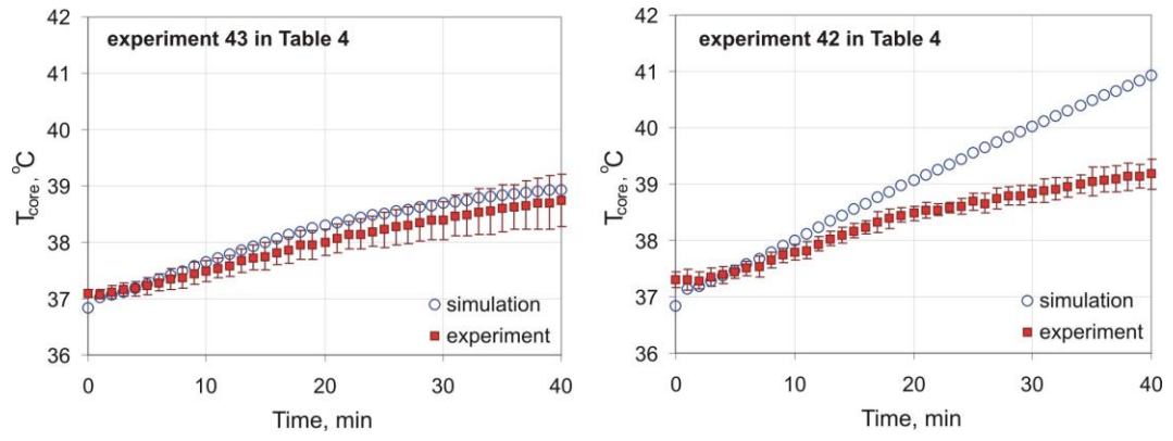
Fig. 16 Body core temperature (rectal) ( T_{core} ) predicted and measured in untrained subjects (exp. 43 in Table 4) and in professional sportsmen (exp. 42 in Table 4) exercising at 90% of their individual anaerobic threshold corresponding to metabolic rates of 9.2 met and 12.0 met, respectively
