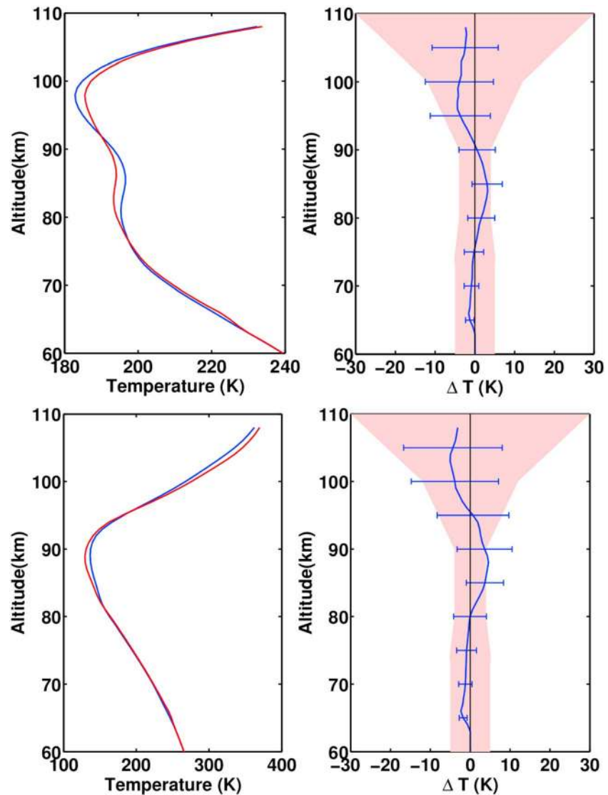
Figure 3. (top left) Comparison of the March and September mean vertical profile from SABER operationally retrieved v2.0 kinetic temperature (blue line) and the simultaneously retrieved SABER T_k/\text{CO}_2 kinetic temperature (red line). (bottom left) The same comparison as before but for the January and July mean summer hemisphere (see text). (right column) The associated mean differences are in blue color with the standard deviation of the differences indicated as error bars. The combined uncertainty of the two retrievals is shown as a shaded area in Figure 3 (right column).
