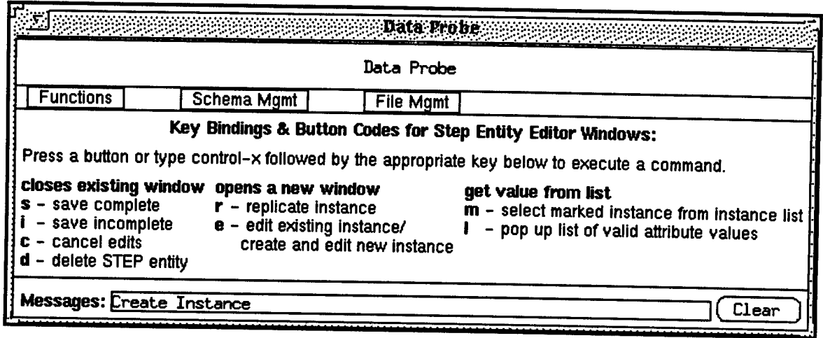
FIGURE 9 Data Probe Management Window
