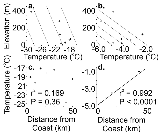
Figure 13. For period of common record at all stations, relationship between (a) elevation and mean annual temperature (for each station, average of all mean annual temperatures that can be calculated between 13 November 1998 and 6 April 2000), (b) elevation and summer temperature (average of temperatures for 1998/1999 and 1999/2000 summers), (c) distance from coast and annual temperature normalized to sea level, and (d) distance from coast and summer (DJF) temperature normalized to sea level. Lines in the elevation plots represent the dry adiabatic lapse temperature gradient for reference.
