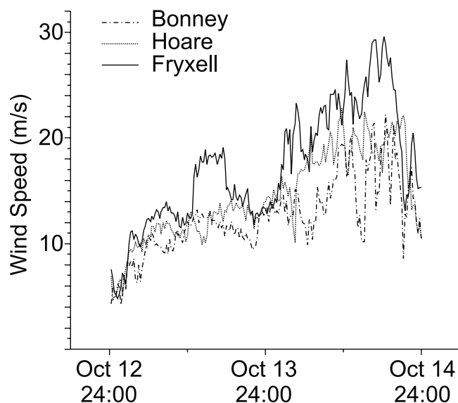
Figure 7. Katabatic event in Taylor Valley during spring 1999. This event produced the highest maximum wind speed in our record.
