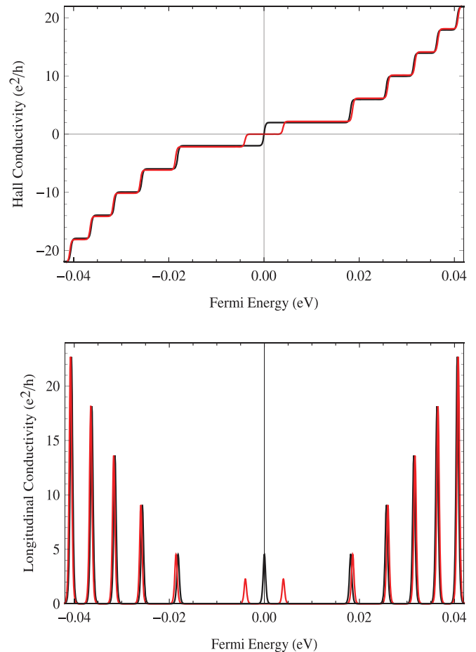
Figure 2 | Hall (top) and longitudinal (bottom) conductivities as functions of the Fermi energy for 0 meV (black line) and 4 meV (red line) SOI energy. T = 2 \text{ K} , \Delta_z = 0 \text{ meV} , and B = 1 \text{ T} . This situation represents a trivial insulator.
