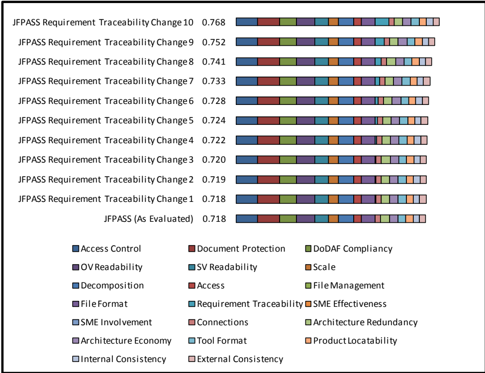
Figure 75. Requirement Traceability Measurement Analysis
