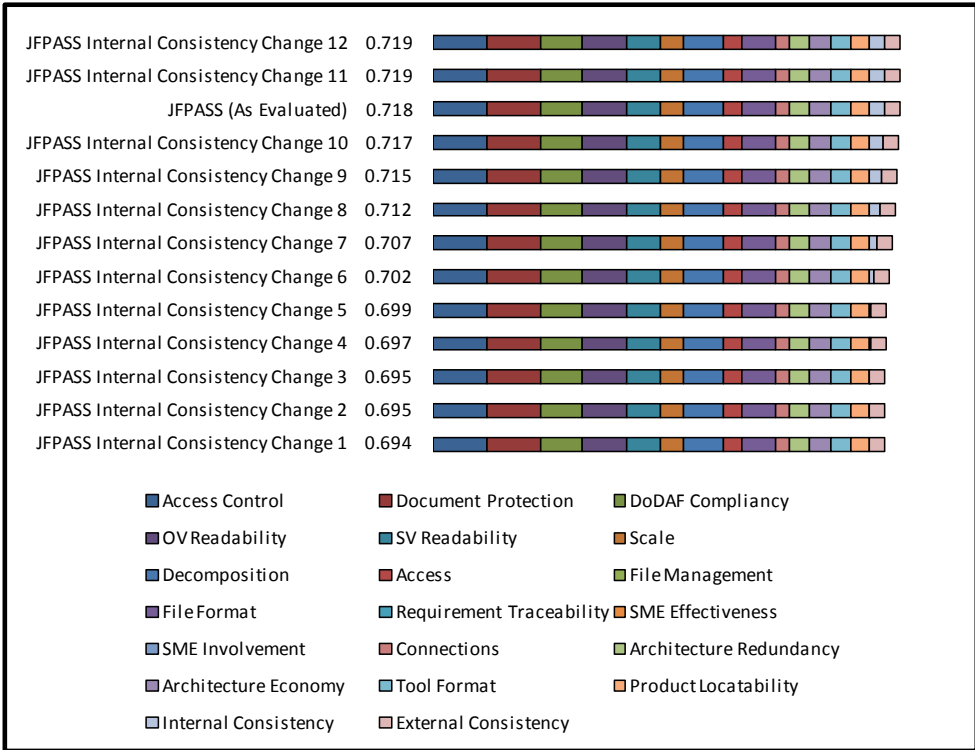
Figure 76. Internal Consistency Measurement Analysis
