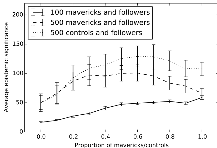
Fig. 2 EL model with cost of exploration. Progress measured as average epistemic significance of the population after 200 time steps.
