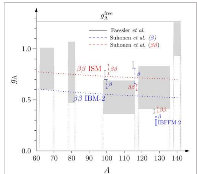
FIGURE 18 | Sketch of the effective values of g_A taken from Table 9 against the light-hatched ranges of g_A^{\text{eff}} in the 5 mass regions of Figure 2 (the combined pnQRPA results). The curves are from the 2\nu\beta\beta analysis of Barea et al. [191] [curves (86)] and the vertical segments display the results of the combined \beta and 2\nu\beta\beta analyses of Faessler et al. [188, 189] (solid line) and Suhonen and Civitarese [192] (dashed lines). Also the (combined) IBFFM-2 result of Yoshida and Iachello [190] is depicted.
