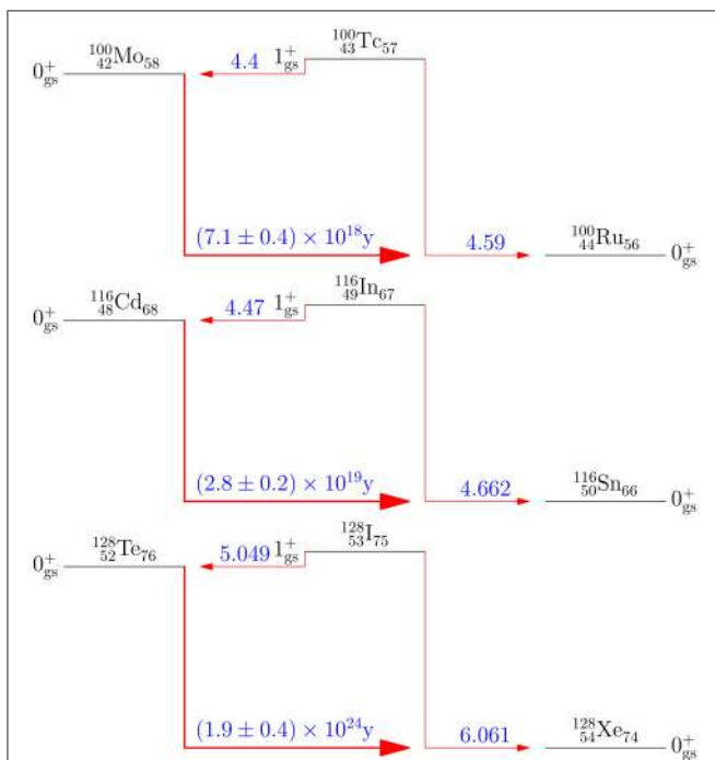
FIGURE 17 | Schematic plot of \beta and \beta\beta decays in the three isobaric chains ( A = 100, 116, 128 ) with data on both decay modes. Given are the 2\nu\beta\beta half-life and \log ft values of the left- and right-branch \beta decays.
