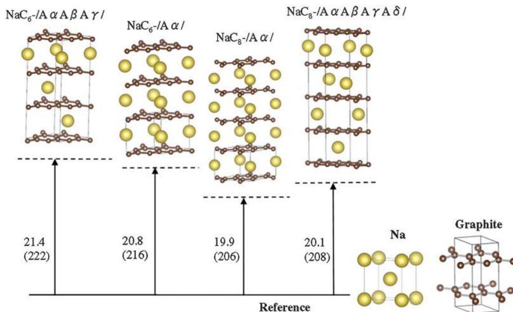
Fig. 5 Illustration of the enthalpy of formation in \text{kJ mol}^{-1} ( \text{meV f.u.}^{-1} ) of first stage Na-GICs relative to the reference state corresponding to pure graphite and Na metal. The compound at the lowest position is the most stable structure. Arrow lengths are not to scale.
