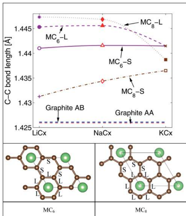
Fig. 9 [Top] In-plane C–C long (L) and short (S) bonds in MC_x intercalation compounds and graphite AB and artificial graphite AA. Configurations of long (L) and short (S) bonds for MC_6 and MC_8 are illustrated in bottom left and right figure respectively.
