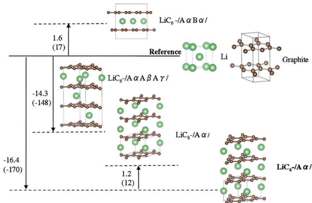
Fig. 3 Illustration of the enthalpy of formation in \text{kJ mol}^{-1} ( \text{meV f.u.}^{-1} ) of first stage Li-GICs relative to the reference state corresponding to pure graphite and Li metal. \text{LiC}_6\text{-}/A\alpha/ is the most stable compound. Arrow lengths are not to scale.
