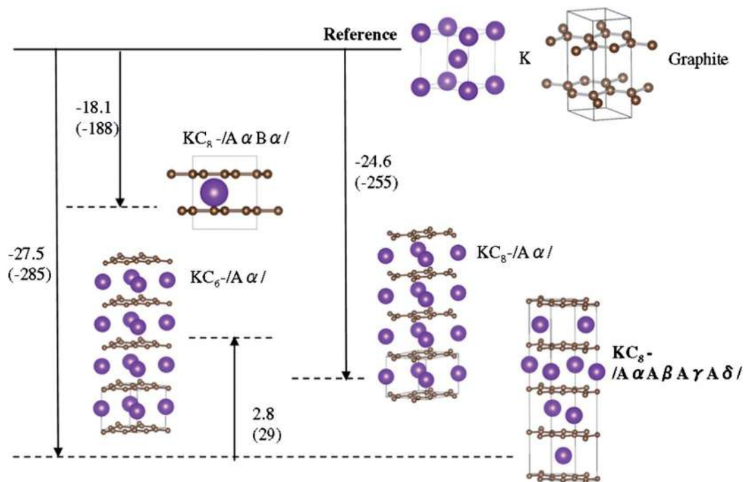
Fig. 4 Illustration of the enthalpy of formation in \text{kJ mol}^{-1} ( \text{meV f.u.}^{-1} ) of first stage K-GICs relative to the reference state corresponding to pure graphite and K metal. The compound at the lowest position is the most stable structure. Arrow lengths are not to scale.
