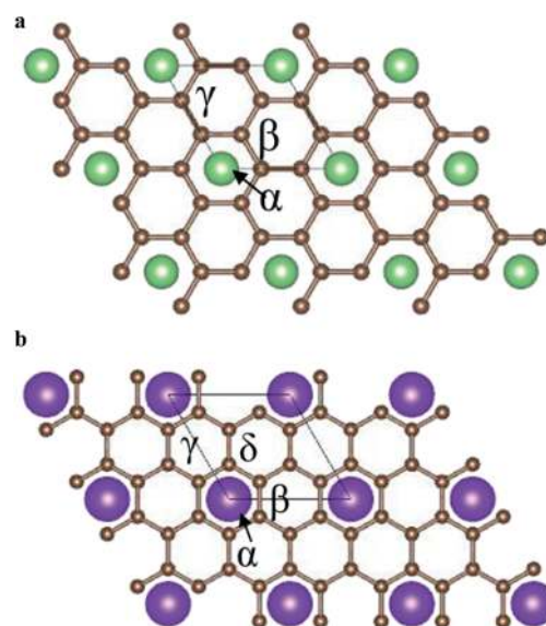
Fig. 2 \text{MC}_6 with in-plane p(\sqrt{3} \times \sqrt{3})R30^\circ structure (a) and \text{MC}_8 with in-plane p(2 \times 2)R0^\circ structure (b). Carbon is represented by brown spheres, while the spheres with the other colours represent alkali metals. 77 \alpha , \beta , \gamma and \delta represent the equivalent intercalation sites.
