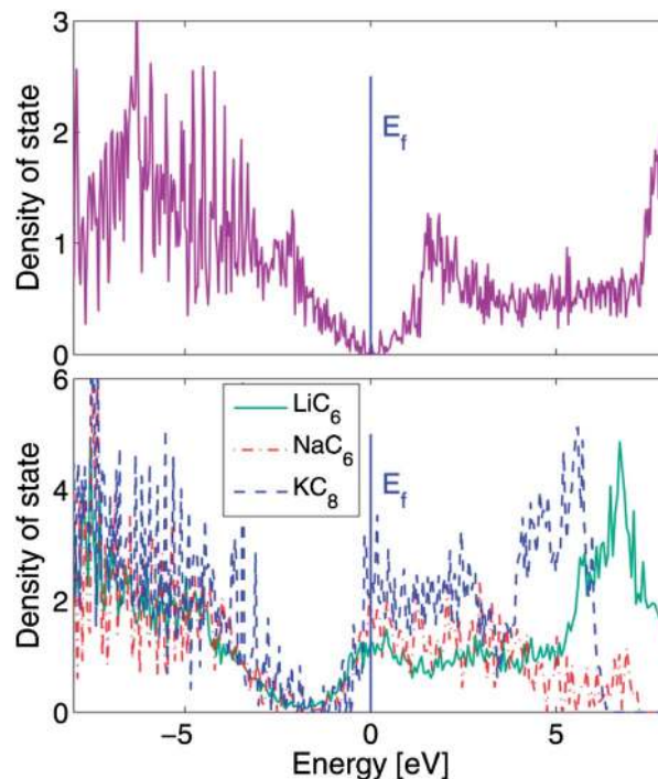
Fig. 10 Total DOS of graphite (top) and MC_x intercalation compounds (bottom).
