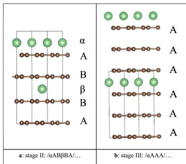
Fig. 6 Structures of stage II and III Li-GICs. Brown balls represent carbon atom and green balls represent Li metal.
