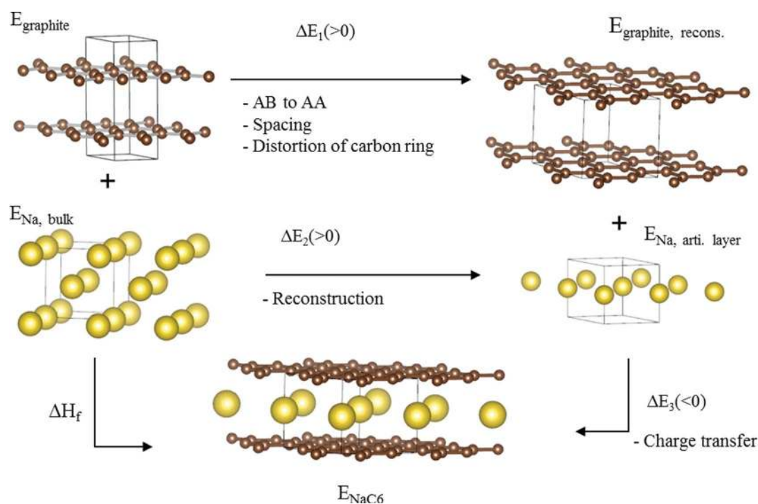
Fig. 12 The hypothetical reaction cycle for the formation of AM-GICs from the elements using NaC 6 as an example. \Delta E_1 and \Delta E_2 correspond to the energy required for the reconstruction of graphite and alkali metal into the layers corresponding to the intercalation compound. \Delta E_3 corresponds to the energy gain from the charge transfer when the artificial alkali metal layer intercalates the carbon host.
