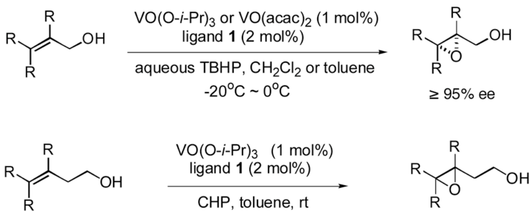
Scheme 1. Asymmetric epoxidation of allylic alcohols and homoallylic alcohols by vanadium and BHA complex.
