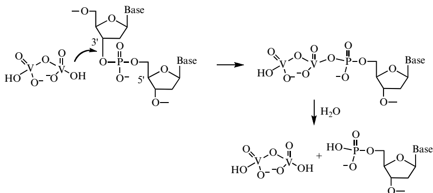
Figure 7 Proposed mechanism for the pyrovanadolysis of the DNA primer [36]: Divanadate attacks the primer at the 3' position, a process which affords mediation by Mn^{2+} . The transiently formed 3'-divanadophospho-nucleotide is hydrolytically split into divanadate and the phosphonucleotide to which DNA polymerase falls back.
