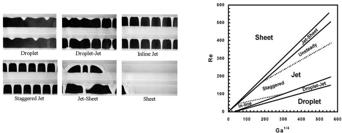
Figure 1: The falling-film modes between horizontal tubes and flow regime map of Hu and Jacobi, 1996a, 1996b.
