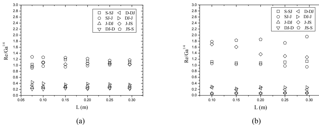
Figure 5: Liquid feeding length effects on falling-film mode transitions. (a) is for water, Ga^{1/4} \approx 429 ; (b) is for ethylene glycol, Ga^{1/4} \approx 17 , and s/d = 0.95 . These data were obtained with a quiescent gas.
