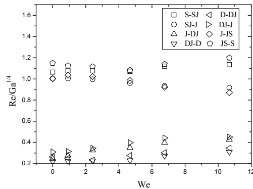
Figure 6: Vapor-shear effects on falling-film mode transitions, Ga^{1/4}=465 (Water), s/d=0.95, s/a=8.82, L=0.1\text{m} .
