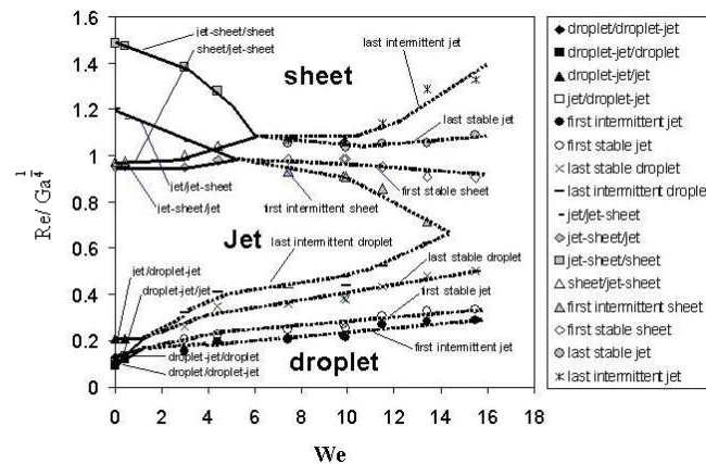
Figure 2: Vapor shear effects on falling-film mode transitions, Ga^{1/4}=35.7, s/d=1, s/a=9.3 (Wei and Jacobi, 2002)
