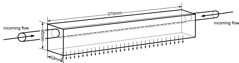
Figure 4: Feeding system design
