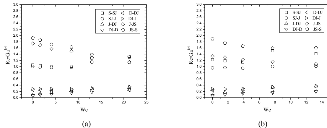
Figure 8: Vapor-shear effects on falling-film mode transitions at different liquid feeding lengths, (a) L=0.1\text{m} , (b) L=0.295\text{m} , Ga^{1/4} \approx 17 (Ethylene Glycol), s/d=0.95 , s/a=11.4 .
