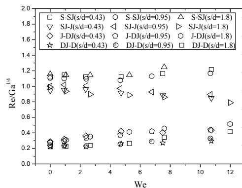
Figure 7: Vapor-shear effects on falling-film mode transitions with different geometry factor s/d , without considering hysteresis effect, Ga^{1/4}\approx 450 (Water).
