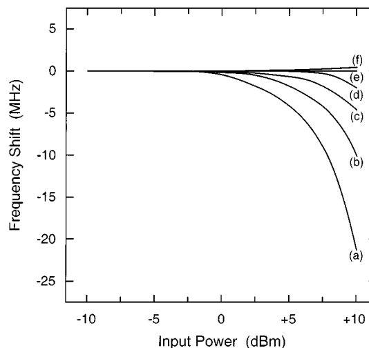
Fig. 9. Measured shift in notch position as a function of input drive level for nominal notch positions at: (a) 9.5 GHz, (b) 9.625 GHz, (c) 9.75 GHz, (d) 9.875 GHz, (e) 10 GHz, and (f) 10.125–10.5 GHz.
