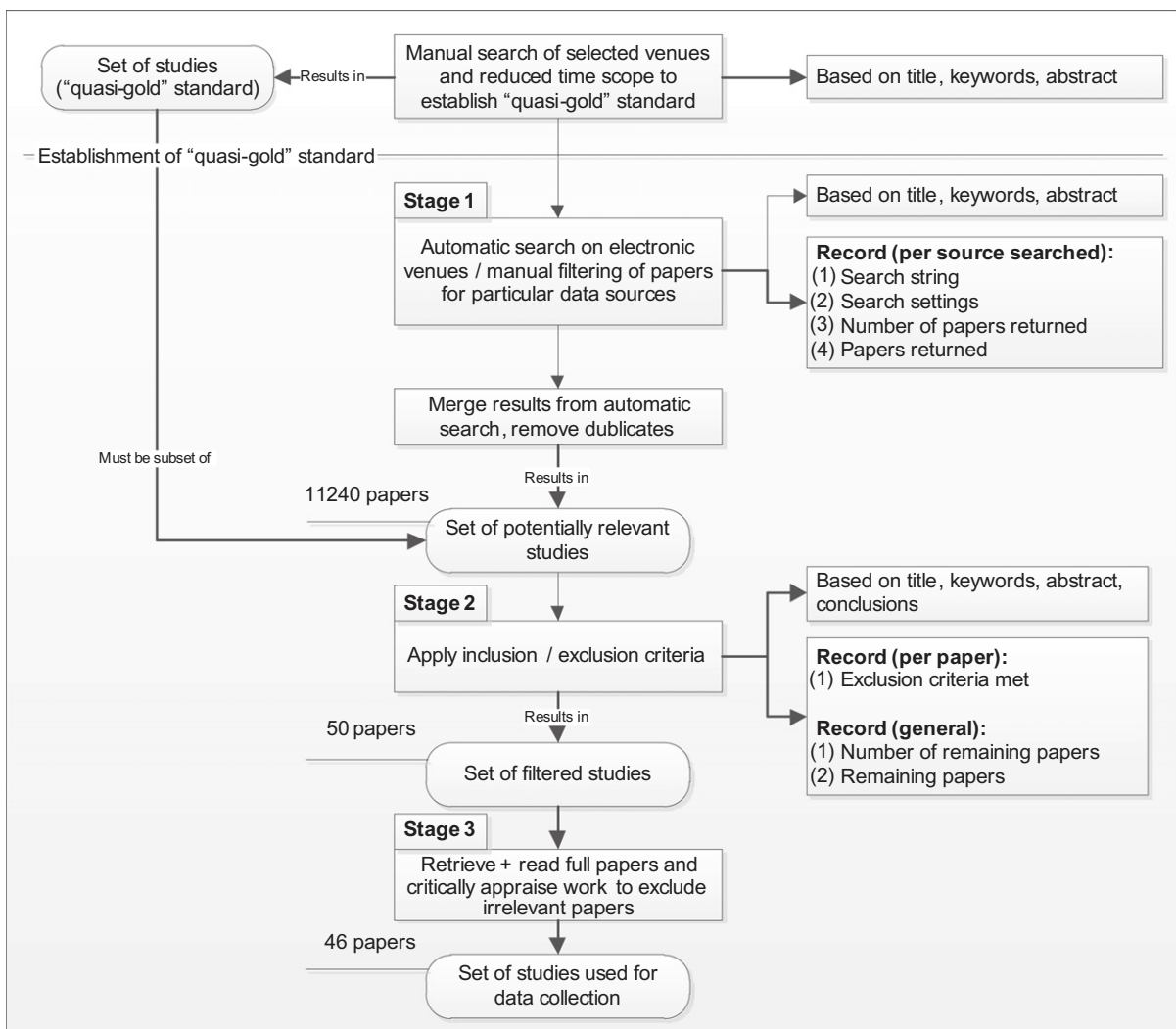
Fig. 2. Search process.
