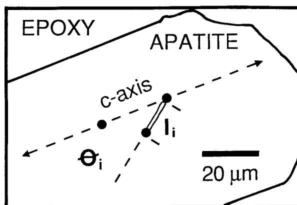
FIGURE 2. Fission-track length ( l_i ) and inclination angle ( \theta_i ) to the crystallographic c axis.
