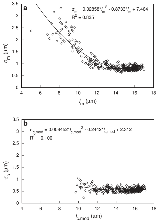
FIGURE 9. (a) Plot of \sigma_m vs. l_m for all 387 experiments Carlson et al. (1999, this volume). (b) Plot of \sigma_{c, \text{mod}} vs. l_{c, \text{mod}} for all 387 experiments.
