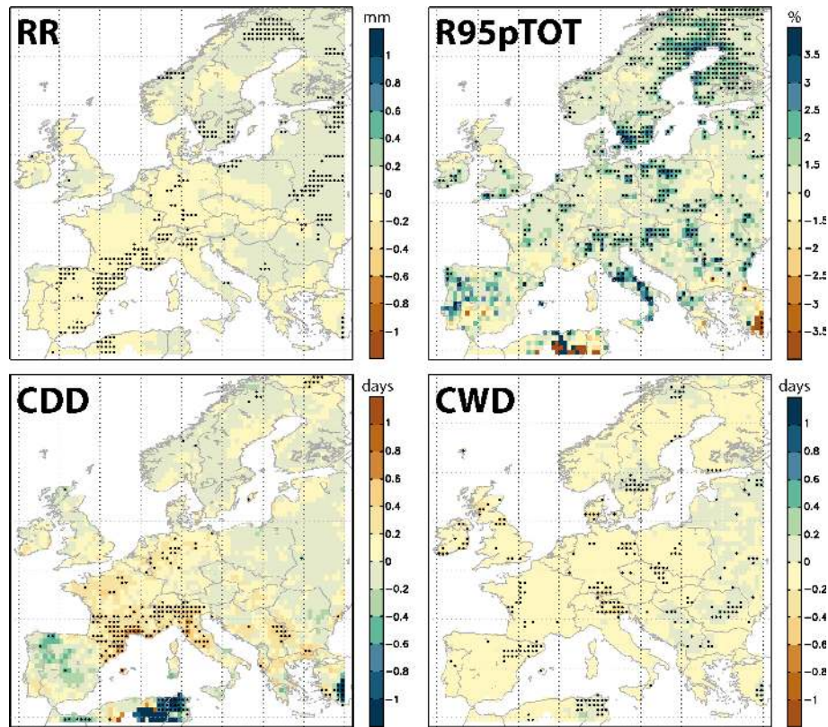
Fig. 6. As in Fig. 2, but for summer.
