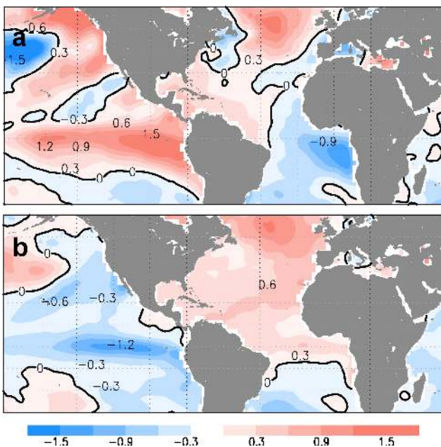
Fig. 11. Composite maps of SST for R95pTOT (PC1) (a) and for the AMO (b) in autumn.
