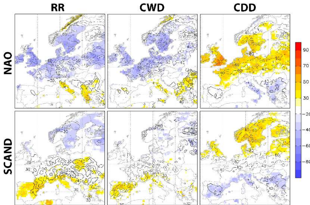
Fig. 7. Shaded regions represent the correlation coefficients ( \times 100 ) between the teleconnection indices (NAO, SCAND, by rows) and the mean or extreme precipitation fields (by columns) in summer. Contour lines represent the EOF associated with the PC better correlated with the teleconnection index according to Table 4.
