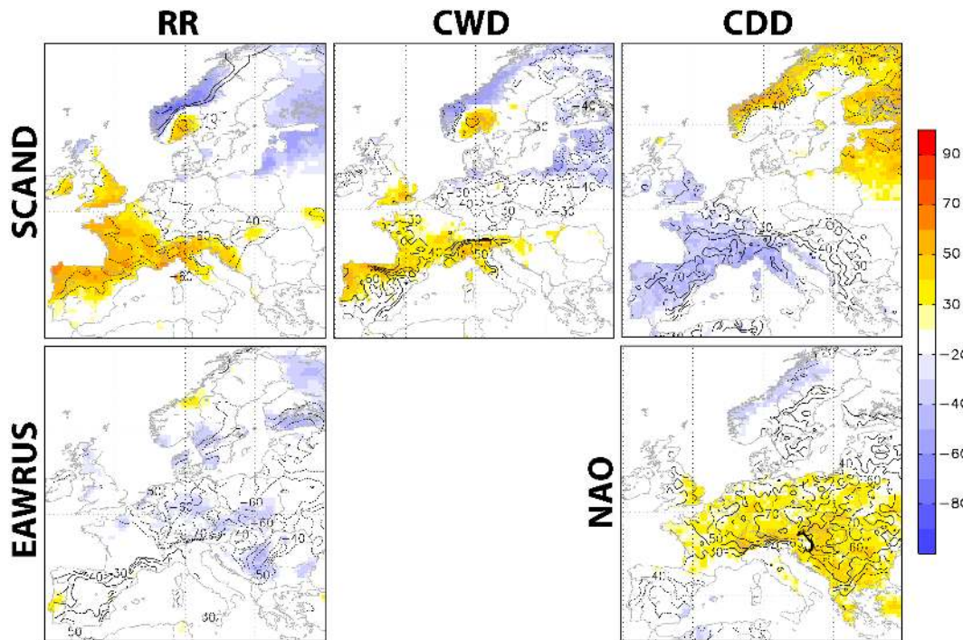
Fig. 10. Shaded regions represent the correlation coefficients ( \times 100 ) between the teleconnection indices (SCAND, EAWRUS, NAO, by rows) and the mean or extreme precipitation fields (by columns) in autumn. Contour lines represent the EOF associated with the PC better correlated with the teleconnection index according to Table 5.
