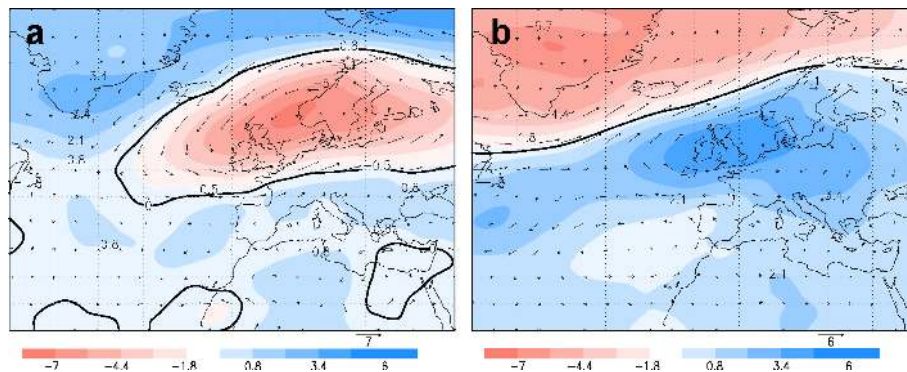
Fig. 8. Composite maps of SLP (hPa) and wind ( \text{m s}^{-1} ) at 850 hPa for CDD (PC2) (a) and for the NAO (b) in summer.
