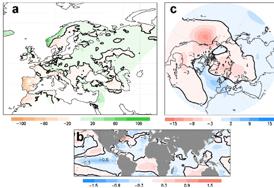
Fig. 5. Composite maps of RR (a), SST (b) and SLP (c) for anomalous MJO phase 3 in winter.
