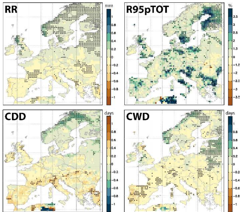
Fig. 2. Trend maps of RR, R95pTOT, CDD and CWD in winter. Shadings represent the Sen's slope per decade (bluish (brownish) colours mean wetter (drier) conditions). The black dots correspond to those points where the trends are statistically significant at 5 % significance level (Z Kendall's coefficient).
