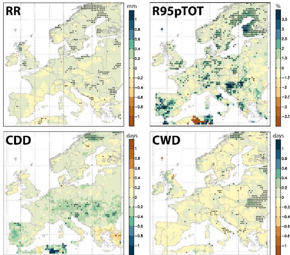
Fig. 9. As in Fig. 2, but for autumn.
