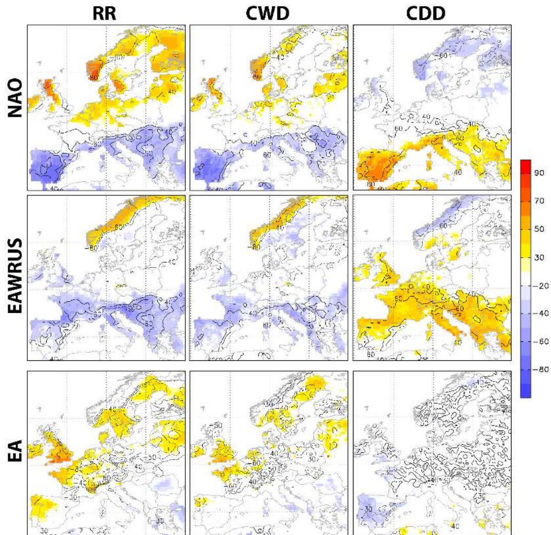
Fig. 3. Shaded regions represent the correlation coefficients ( \times 100 ) between the teleconnection indices (NAO, EAWRUS, EA by rows) and the mean or extreme precipitation fields (by columns) in winter. Contour lines represent the EOF associated with the PC better correlated with the teleconnection index according to Table 2.
