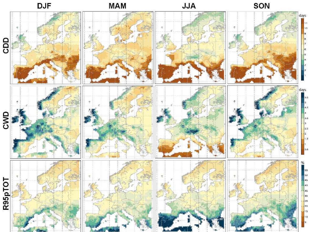
Fig. 1. Seasonal mean distribution of CDD (days), CWD (days) and R95pTOT (%) for the different seasons (columns).
