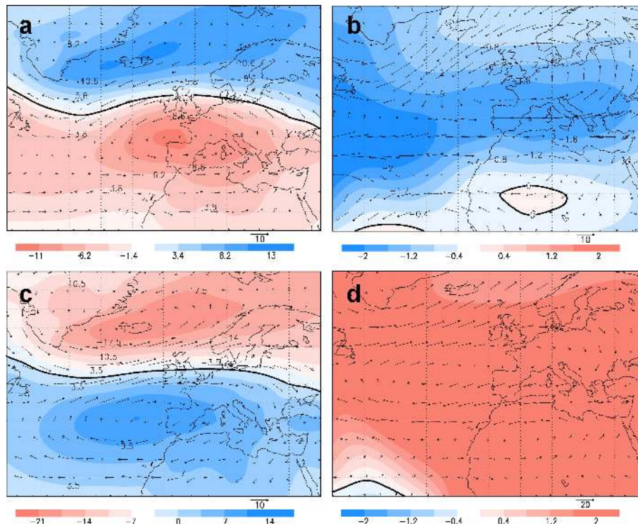
Fig. 4. Composite maps of SLP (hPa) and wind ( \text{m s}^{-1} ) at 850 hPa (a) and velocity potential ( \times 10^6 \text{ m}^2 \text{ s}^{-1} ) at 200 hPa (b) for extreme CWD (PC1) in winter. Same maps for the NAO (c and d).
