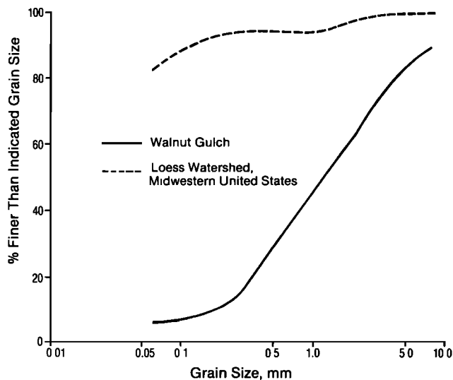
Fig. 4. Particle size analyses for the channels of the main trunk of Walnut Gulch and a typical loess watershed in the midwestern United States.
