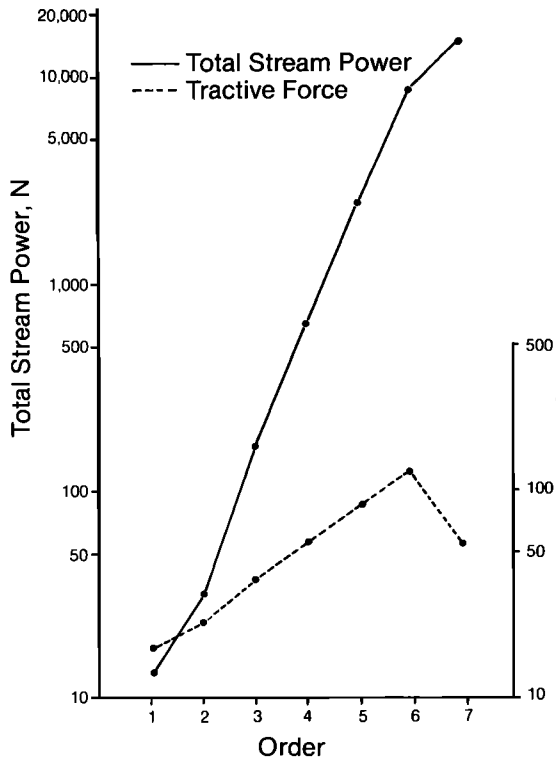
Fig. 9. Distributions by stream order of mean values for tractive force and total stream power for channels of Walnut Gulch Watershed.
