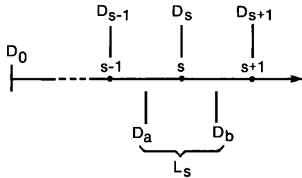
Fig. 3. Schematic diagram defining factors used to calculate volume of sediment transported during the erosion episode on Walnut Gulch.
