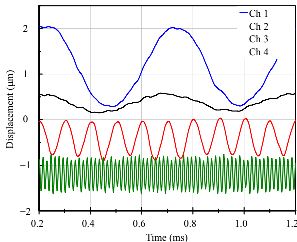
Fig. 9 Demodulated output signals from the 4 targets (the top 2 traces were generated when the B&K shaker was driven at 2 kHz with amplitudes of 0.8 microns (Ch1) and ~0.25 (Ch2) microns, respectively; Channel 3 (third trace from top) was generated when shaker 3 was driven at 10 kHz with amplitude of 0.4 microns and Channel 4 (bottom trace) at 60 kHz with amplitude of ~0.3 microns).
