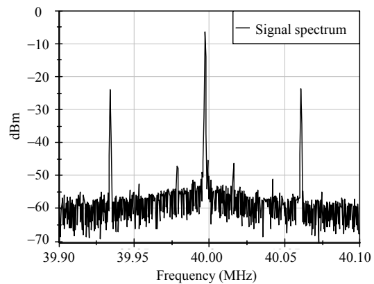
Fig. 11 Spectrum of the carrier modulated with a 60 kHz signal (PZT) measured at a range of 50 m.
