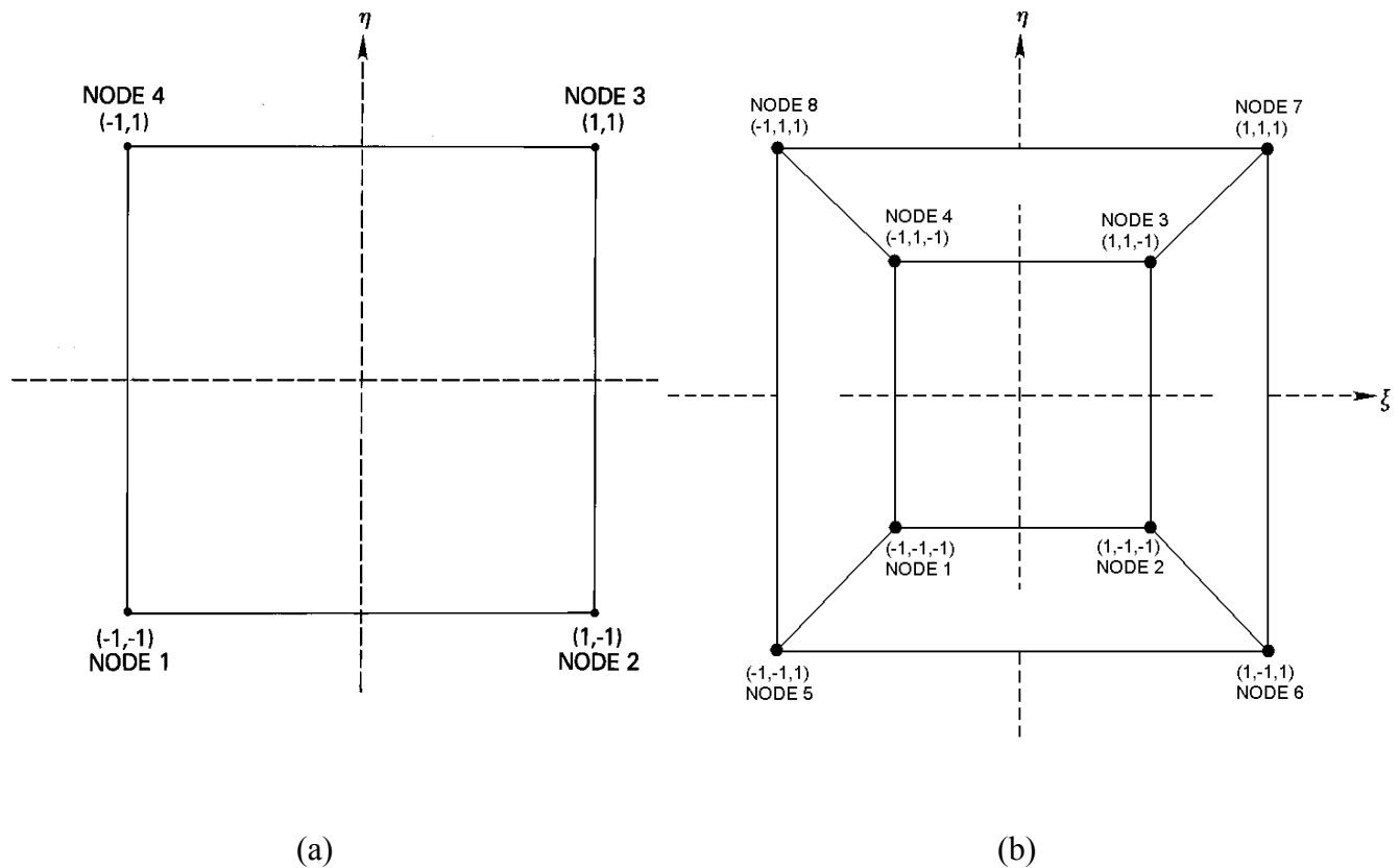
Figure 4.1 . (a) Quadrilateral 2D finite element in local coordinate system (\xi, \eta) . (b) Hexahedral 3D finite element in local coordinate system (\xi, \eta, \zeta) . The \zeta -axis points directly out of the page.
