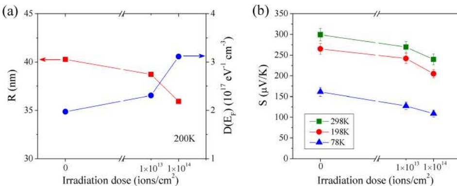
FIG. 4. Properties of a BP nanoribbon before and after He ^{2+} irradiation. (a) Irradiation dose dependence of average hopping distance and density of states of traps at the Fermi level at 200 K. (b) Irradiation dose dependence of Seebeck coefficient at 298 K, 198 K, and 78 K.
