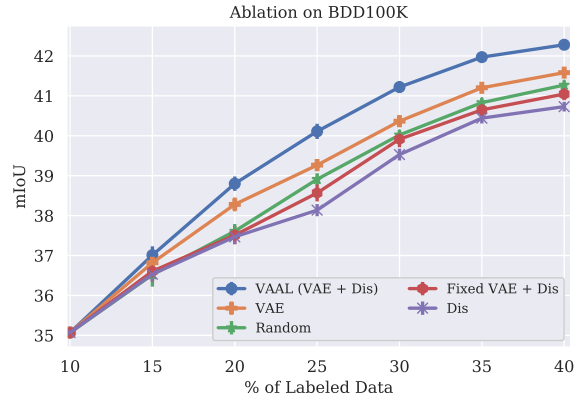
Figure 4. Ablation results on analyzing the effect of the VAE and the discriminator denoted as Dis here,
