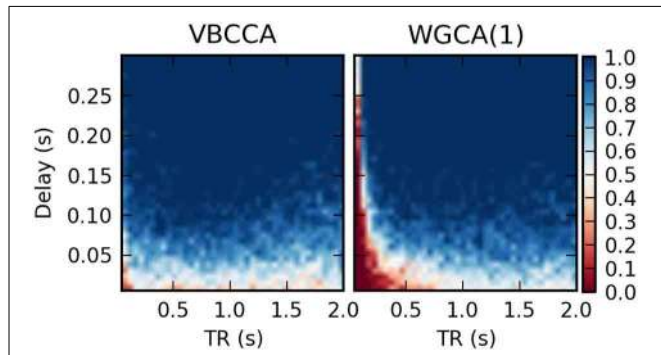
FIGURE 9 | Average d-Accuracy calculated over 50 simulations for a network with two nodes and a single connection for varying neuronal delays (40 steps between 5 and 300 ms) and TR values of the fMRI scanner (40 steps between 50 ms and 2 s). The HRF is held constant for all simulations, the signal-to-noise ratio is 20 dB. The proposed method is denoted VBCCA and we use P = 1 , whereas WGCA(1) denotes the Wiener–Granger causality method, for which we also use AR model order of 1.
