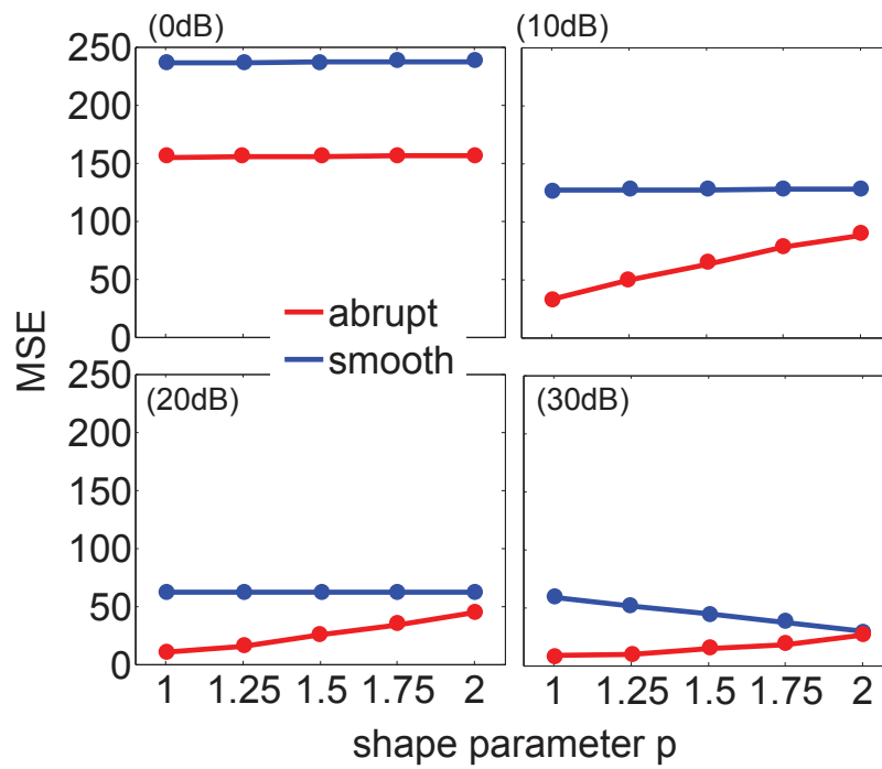
Fig. 3. Quantification of the algorithm performance. From very high (SNR=0dB) to very low noise (30dB), the MSE between the original sources and the final estimates is plotted versus the prior shape parameter p . Concretely we have simulated p = 1.00, 1.25, 1.50, 1.75, 2.00 . Red lines are corresponding to the MSE obtained for abrupt sources and the blue lines are for the smooth situation.
