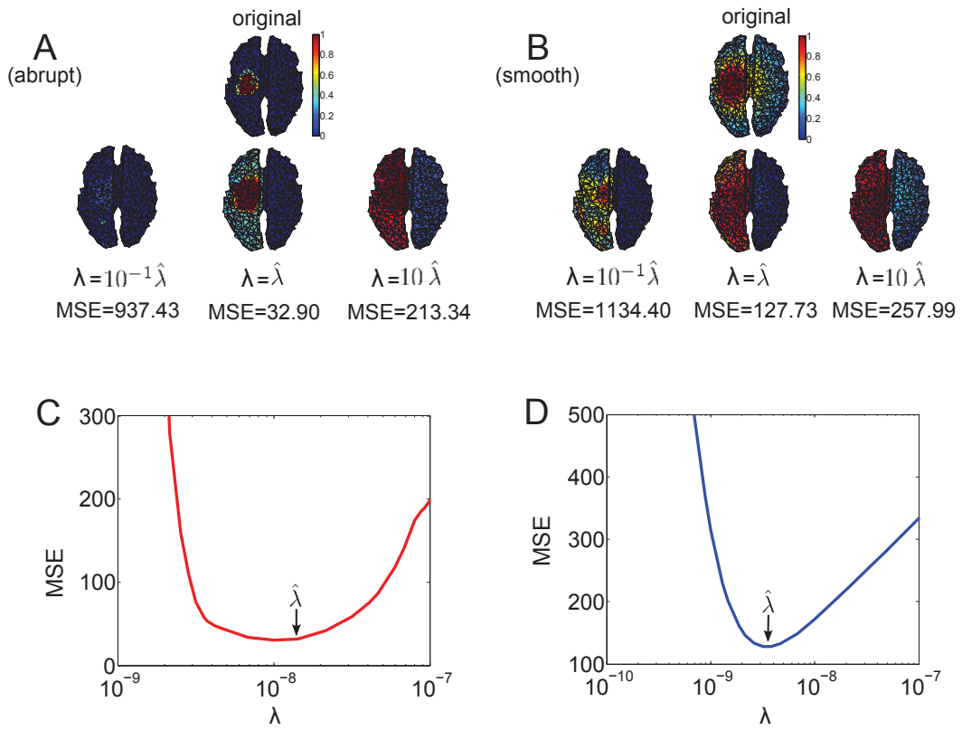
Fig. 4. Validation of the hyperparameter estimation. A,C: Abrupt sources and p = 1 . B,D: Smooth sources and p = 2 . A,B: Brain activity visualization for the original and the final estimates at different values of the hyperparameters ratio \lambda \equiv \alpha/\beta (details in the text). The value of \lambda = \hat{\lambda} is the one corresponding to the algorithm estimation, marked with an arrow in panels C (abrupt) and D (smooth). For illustration purposes, we also showed the final estimates and their corresponding MSE localization values for values of \lambda = 10\hat{\lambda} and \lambda = 10^{-1}\hat{\lambda} . C,D: For both panels, the algorithm estimation performs close to the minimum of the MSE curve. A,B,C,D: Noise was fixed to SNR=10dB.
