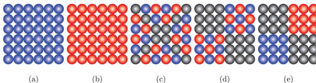
Figure 5. Homogeneously (a and b) and heterogeneously (c, d, and e) charged plates. Blue means a positive charge 0.2 e . Red means a negative charge -0.2 e . Gray means neutral.
