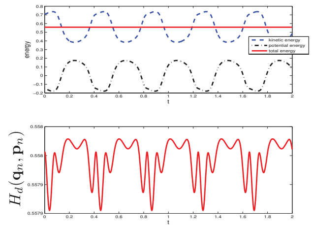
Fig. 17 (online colour at: www.zamm-journal.org ) Six-body linkage: energy in terms of (q_n, q_{n+1}) and (q_n, p_n) (symplectic-momentum scheme, h = 10^{-3} ).
