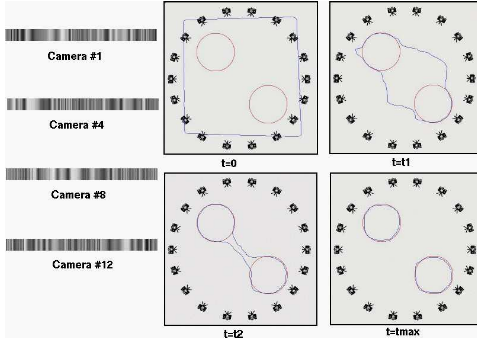
Figure 6: 2D case – Detection of two circular objects.
