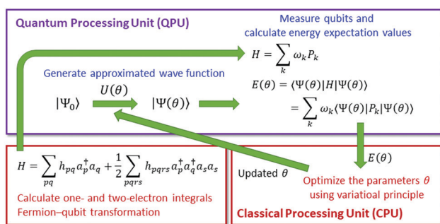
Fig. 2 A schematic view of the VQE-based quantum chemical calculations.
