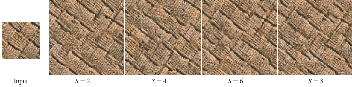
Fig. 7 Synthesis results with different sparsity S = 2, 4, 6, 8 . His example illustrate the artifacts caused by the superposition of several atoms for larger S .
