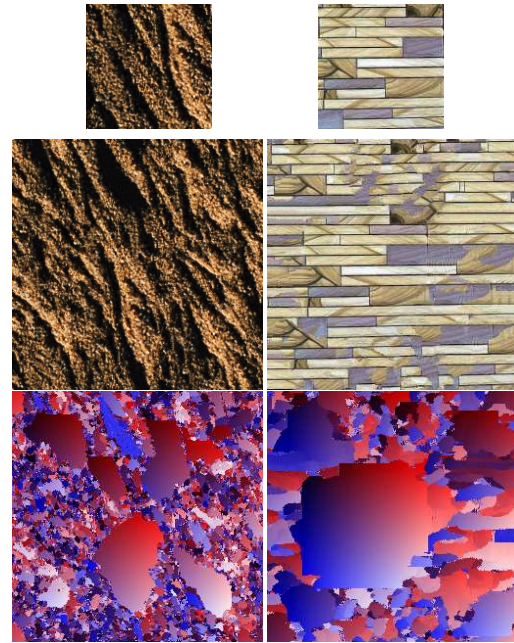
Fig. 3 Results from the pixel-by-pixel copy-paste algorithm [8] (middle); the coordinate maps (bottom) show that the results are tilings from the exemplars (top), even if the synthesis is performed pixel after pixel
