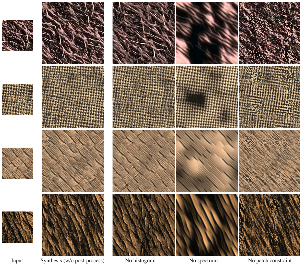
Fig. 4 Synthesis results when dropping one of the three terms. The histogram term prevents from a loss of contrast. The spectrum term spatially regularizes the synthesis and generates granularity. The patch decomposition term handles sharp edges. Note that the post-process is not performed to allow a fair comparison of each term.
