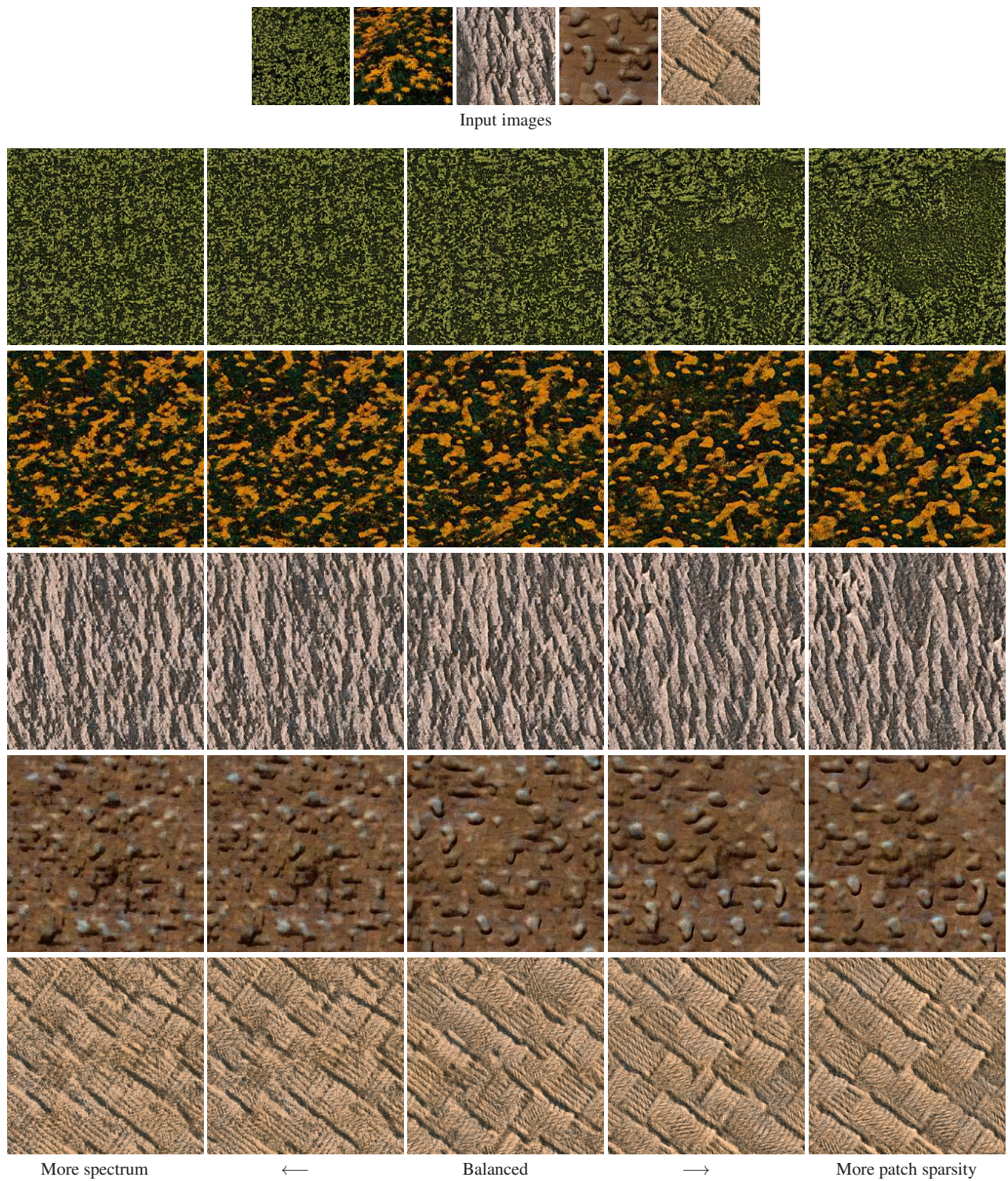
Fig. 6 Synthesis results with different weighting: more spectrum on the left, more patch sparsity on the right. Textures with few geometrical content (top) are better reproduced with more spectrum; textures with large structures (bottom) need more patches sparsity.
