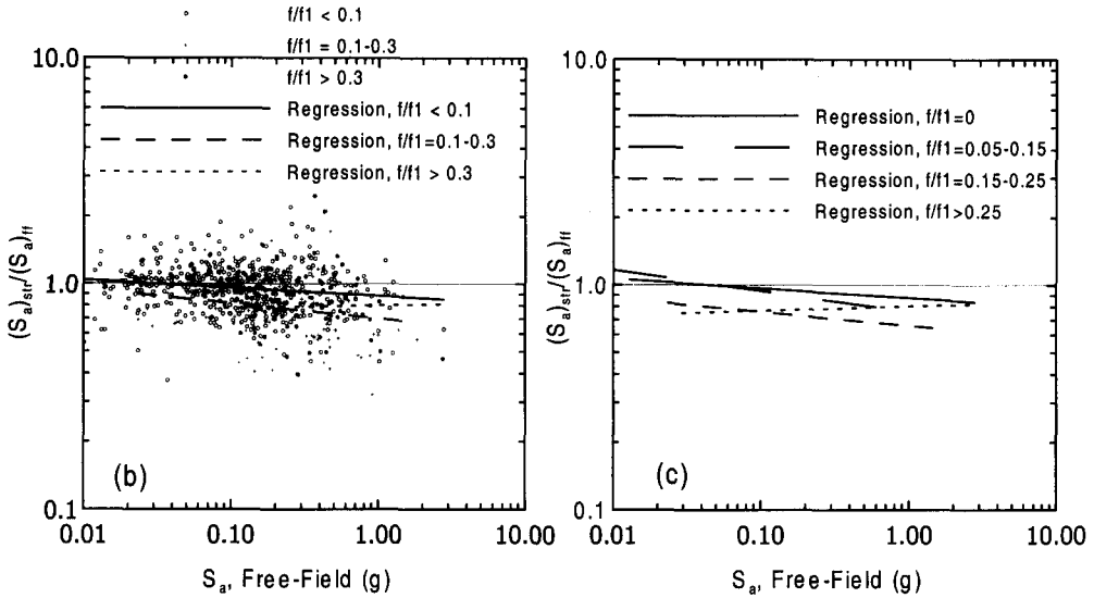
Figure 3(b-c). Ratio of foundation-level/free-field motion, complete data set, sorted by fff_1 .
