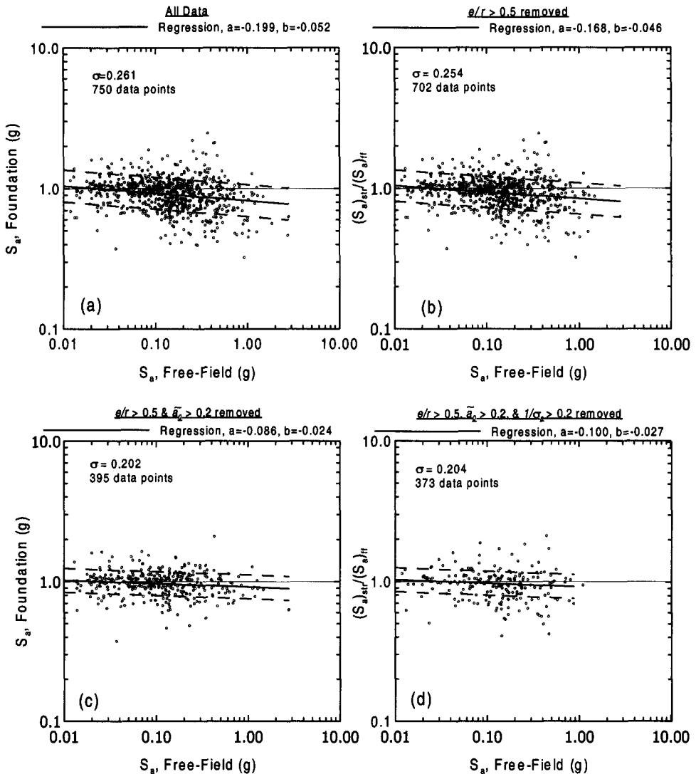
Figure 6. Summary of foundation/free-field ratios of 5% damped spectral accelerations, sorting by e/r , \bar{a}_0 , and 1/\sigma_s .
