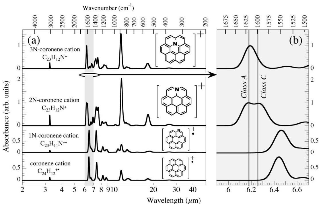
FIG. 3.—Calculated IR spectra of the three possible N-substituted coronene cations compared to that of the parent (unsubstituted) hydrocarbon. (a) Complete spectrum from 2 to 50 \mu\text{m} . (b) Blowup of the 6 \mu\text{m} region of each spectrum. The average positions of the interstellar class A and class C 6.2 \mu\text{m} emission components (Peeters et al. 2002) are indicated in (b), shifted to compensate for the \sim 10\text{ cm}^{-1} redshift difference between emission and absorption peak frequencies (§ 2). Note that the coronene cation and the exoskeletal 1N-coronene cation have radical electronic structures (denoted with a dot), while the endoskeletal 2N- and 3N-coronene cations have the more favorable closed-shell structures. All spectra are normalized to the intensity of the strongest band in the 6.2 \mu\text{m} region.
