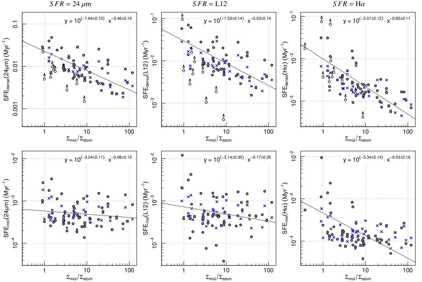
Figure A2. SFE_{\text{dense}} (top row) and SFE_{\text{mol}} (bottom row) as a function of the molecular-to-atomic ratio. From left to right, the SFR is derived from the 24 \mu\text{m} emission, a linear combination of 24 \mu\text{m} and H \alpha intensities (L12), and the H \alpha emission.
