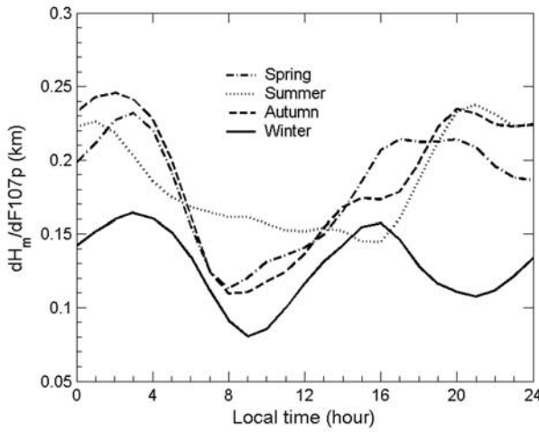
Figure 9. Same as Figure 4, but for the rate of change d(H_m)/d(F_{10.7p}) .
