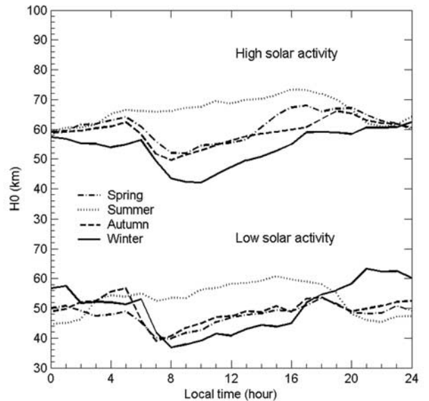
Figure 10. Diurnal and seasonal variations of effective topside scale heights H_0 under low and high solar activities.
