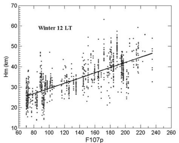
Figure 8. An example of the variation of scale height H_m with solar flux index F_{10.7p} . The solid line is the results from linear regression.
