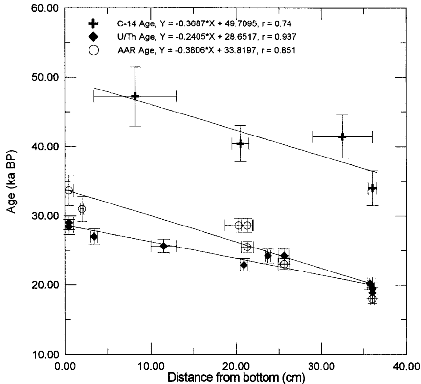
Figure 8 Results of ^{14}\text{C} , U/Th, and AAR dating of speleothem JW2. Samples were taken from different distances from the bottom. Straight lines are linear approximations of results by the least squares method (note the equation lines).
