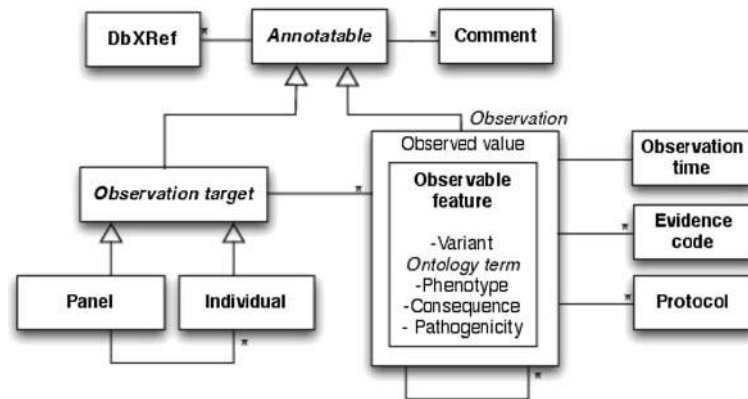
Figure 1 Simplified conceptual UML object model used in VarioML. The VarioML object model is derived from Observ-OM ( http://www.observe-om.org/wiki/ObservStart ), with some modifications to simplify implementation. E.g., Observable Feature (such as phenotype or mutation name ) and Observed Value (existence of phenotype or variation) are denormalized into a single XML element. This avoids unnecessary nesting of observation elements which do often have one-to-one relationship, in the XML implementation. Entities are composed into Observations , having properties such as evidence codes , observation protocols and observation time . Associations between elements are described as single lines, where an asterisk means a 0-to-many multiplicity relationship; i.e. Observation can have one or many evidence codes. All entities also inherit from Annotable properties which are needed for database cross references and comments. In this case, the open arrow symbol means inheritance or an is-a relationship.
