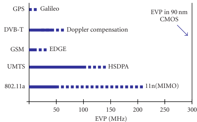
FIGURE 9: Estimated EVP 16 load numbers for the modem stage of various receivers.
