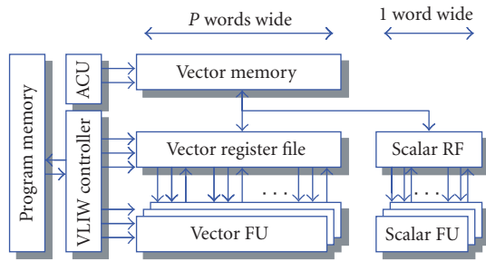
FIGURE 6: A generic vector-processor architecture.
