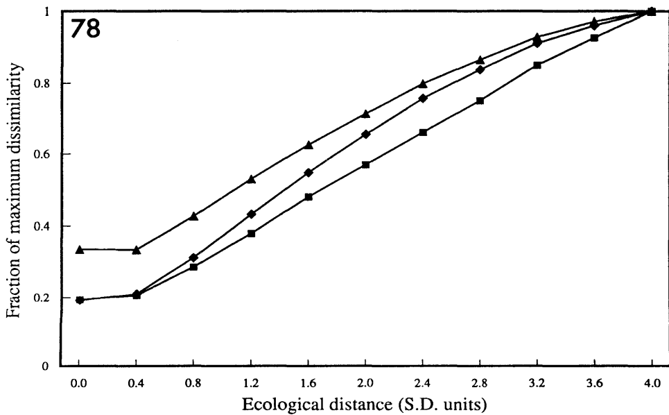
Figs 77-78. Relative ecological distances (in per cent of distances between sample plots 1, respective, 4 S.D. apart) as functions of coenocline separation. Percentage cover data weighted to range 2.5 (after R. Økland 1986a). PD - percentage dissimilarity, Compl. SR - complemented similarity ratio, ED - Euclidean distance divided with the number of species in the two compared sample plots. Fig. 77. Simulated coenocline with length 2 S.D. Fig. 78. Simulated coenocline with length 8 S.D.
