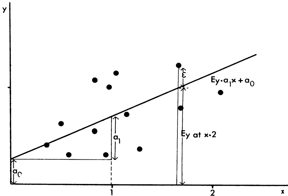
Fig. 80. Geometric interpretation of the parameters of the linear response model. Ey is the systematic part of the model, \epsilon represents the error. a_0 and a_1 are parameters of the regression. For further information, see text.
