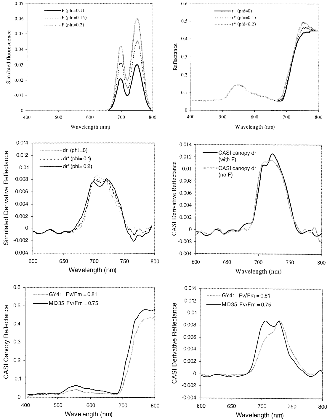
Fig. 3. Simulated leaf reflectance including the effects of fluorescence using the fluorescence–reflectance–transmittance (FRT) model (top and middle left plots) and compact airborne spectrographic imager (CASI) reflectance in the laboratory (middle right plot) and from an airborne campaign (bottom two plots). Top left plot shows simulated fluorescence emission for different values of \phi (ranging from 0 to 0.2), and superimposed on leaf reflectance (top right plot) with peaks at 695 nm ( B_L = 30 nm) and 750 nm ( B_H = 40 nm), N = 1.5 , and C_{a+b} = 40 \mu\text{g}/\text{cm}^2 . Derivative reflectance (middle left plot) for different fluorescence simulations shows a double peak as function of fluorescence emission. Laboratory CASI reflectance from sugar maple seedlings with and without fluorescence emission shows that such effects are captured on the derivative reflectance (middle right plot). Airborne CASI data collected over 30 \times 30\text{-m} sugar maple study sites (bottom plots) from the two sites with highest field-measured F_v/F_m and C_{a+b} (GY41, F_v/F_m = 0.81 ; C_{a+b} = 38.8 \mu\text{g}/\text{cm}^2 ) and lowest (MD35, F_v/F_m = 0.75 ; C_{a+b} = 19.08 \mu\text{g}/\text{cm}^2 ) show comparable double peak features.
