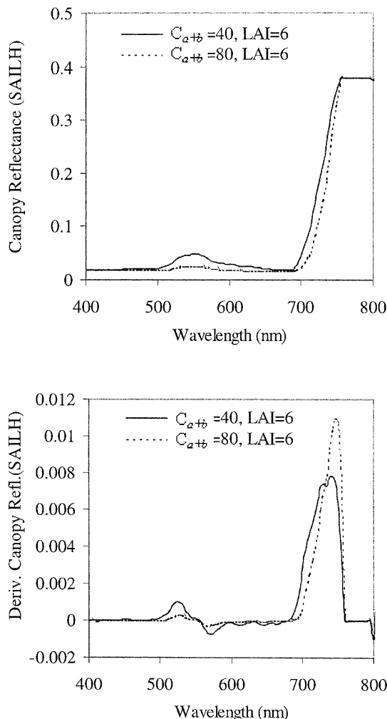
Fig. 4. Simulated canopy reflectance (top) and derivative reflectance (bottom) using the PROSPECT and SAILH radiative transfer models for leaf C_{a+b} = 40 and 80 \mu\text{g}/\text{cm}^2 , N = 1.5 , and canopy leaf area index (LAI) = 6, plagiophile leaf angle distribution function, and nadir view.
