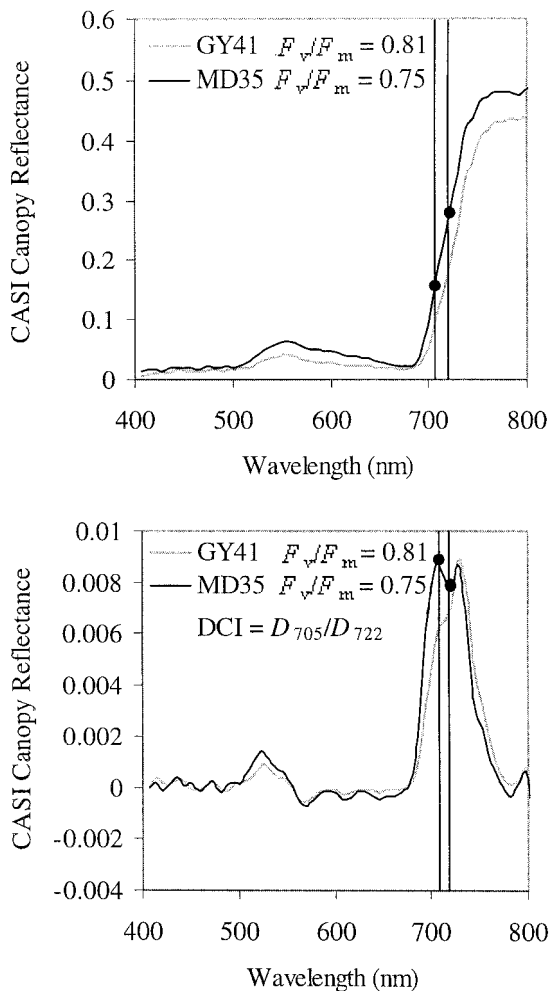
Fig. 5. Band location of the derivative chlorophyll index (DCI) calculated as D_{705}/D_{722} , developed to track changes due to the double peak generated by the suggested effects of pigment and chlorophyll fluorescence at the canopy level in stressed vegetation (healthy site, GY41: F_v/F_m = 0.81 ; C_{a+b} = 38.8 \mu\text{g}/\text{cm}^2 ; stressed site, MD35: F_v/F_m = 0.75 ; C_{a+b} = 19.08 \mu\text{g}/\text{cm}^2 )
