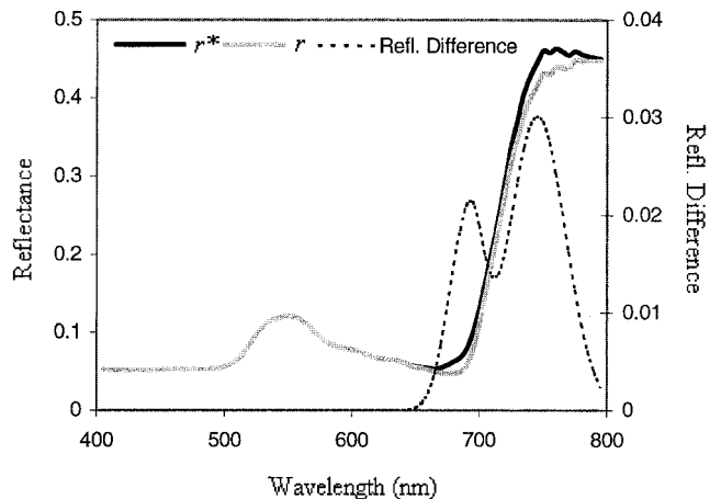
Fig. 2. Fluorescence–reflectance–transmittance (FRT) model simulation of leaf reflectance with the effects of fluorescence flux. Parameters used for the simulation: \phi = 0.085 , C_{a+b} content = 50 \mu\text{g}/\text{cm}^2 , DL = 0.075 \text{ mm} , F_L = 688 \text{ nm} , B_L = 30 \text{ nm} , F_H = 746 \text{ nm} , B_H = 52 \text{ nm} , f ratio F_H/F_L = 0.94 , labeled as r^* (with fluorescence), r (without fluorescence).
