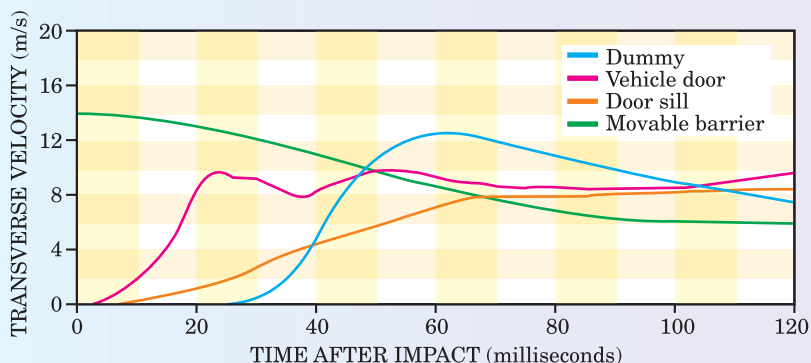
Figure 4. In a side-impact crash test, a moving barrier (green curve) strikes the driver's door of a stationary car at right angles at 31 mph, and then decelerates smoothly to 15 mph. The sill (orange curve) below the door roughly corresponds to the resulting lateral motion of the car as a whole. The rapid intrusion of struck door (red) into the passenger compartment propels the dummy driver (blue) to the right. The maximum acceleration of the dummy's bottom is 70g. (Adapted from ref. 5.)
