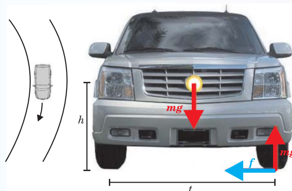
Figure 8. Simplified force diagram for a right turn at the rollover threshold. On a flat road, the vehicle tends to roll toward the outside. About the longitudinal axis through the vehicle's center of gravity, forces on the left front wheel produce a clockwise rollover torque mha and an opposing torque mg t , where h is the height of the center of gravity and t is the distance between front wheels. So if the acceleration a , in units of the gravitational acceleration g , exceeds the stability factor t/2h , the car will roll over.
