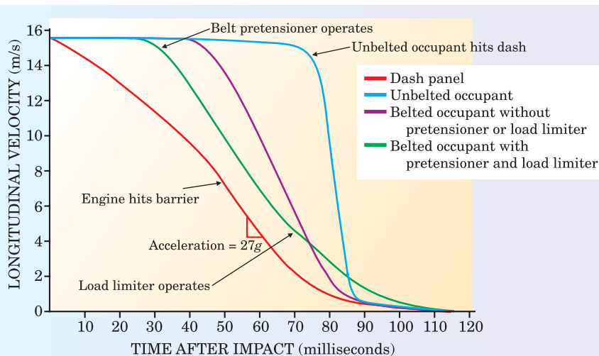
Figure 3. Velocity history of a dummy in the front passenger seat of a car, with various belt restraints, in a 35-mph head-on test crash with a fixed barrier. The red, leftmost curve, representing the car's dash panel, has a maximum deceleration of 27g about 60 milliseconds after impact.
