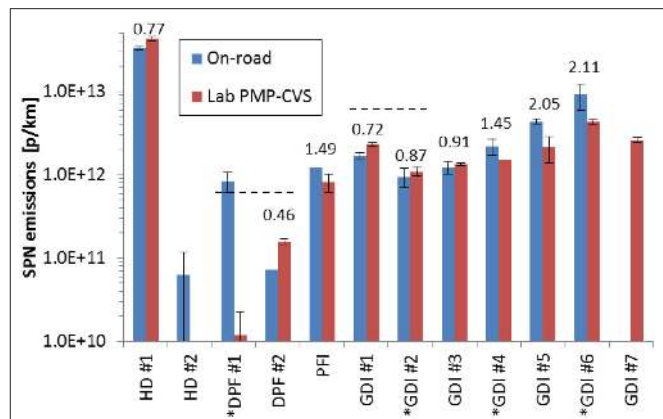
FIGURE 10 | SPN emissions of heavy-duty and light-duty vehicles on the road (PMP-TP) and in the laboratory (PMP-CVS). Asterisk indicates that PEMS-SPN was used instead of PMP-TP system for on-road measurements. DPF regeneration has been excluded from the emission measurements of Vehicles DPF #1 and DPF#2 when tested in the laboratory. On-road results are averages of all tested routes (see Table 3 ). Error bars indicate the range between minimum and maximum SPN emissions. Dashed lines depict the applicable emission limits. Numbers indicate the ratio of on-road to lab emissions.
