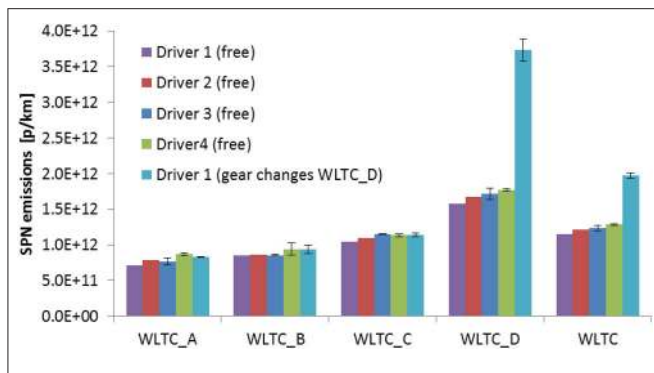
FIGURE 7 | Effect of driving style on the SPN emissions of Vehicle GDI #3. Error bars indicate the minimum and maximum SPN emissions of two test repetitions conducted with 3 months difference between them. All drivers were free to choose their gear shifting, except Driver 1 who followed in one test sequence of WLTC_D a gear shift strategy at higher rpm. Tests in the laboratory were conducted with PMP-CVS equipment.
