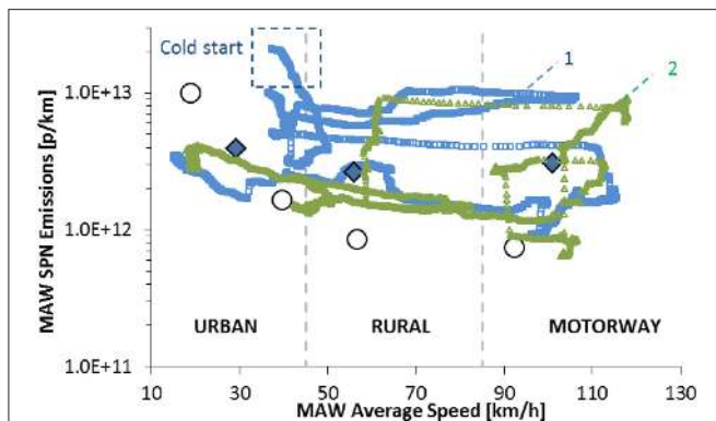
FIGURE 9 | MAW SPN emissions of a road trip with Vehicle GDI #5 in function of the MAW speed. The blue small squares (1) show the first half way of the trip and the small green triangles (2) the return trip. Solid diamonds depict the mean on-road SPN emissions for urban, rural, and motorway driving. White circles depict the laboratory SPN emissions over the four phases of the WLTC.
